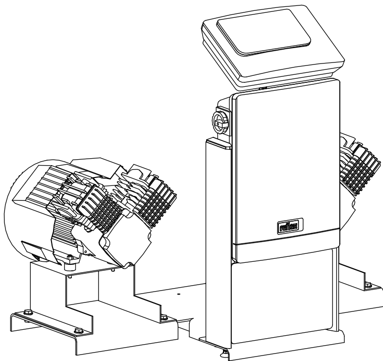
Isometric view
