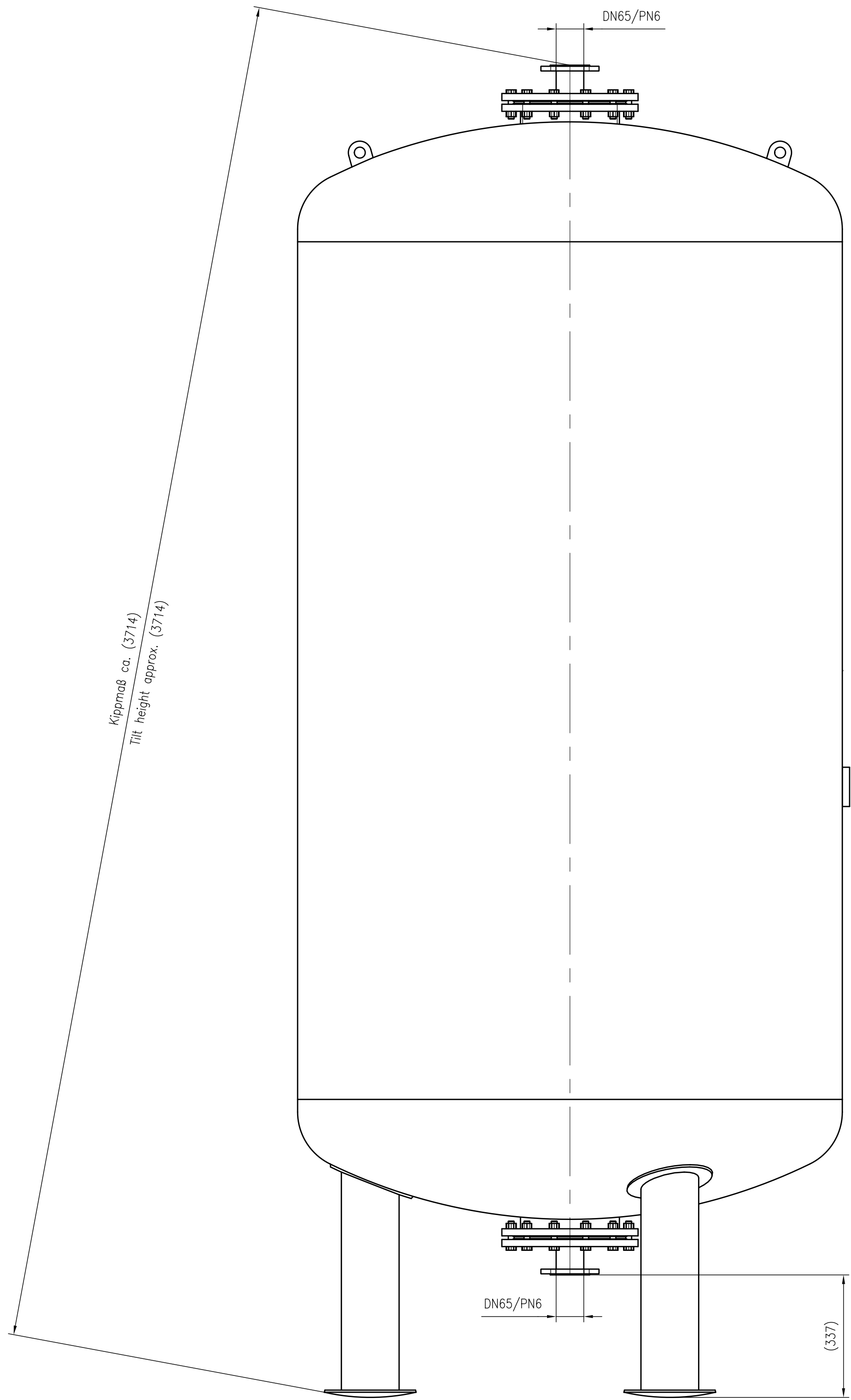
Side view
