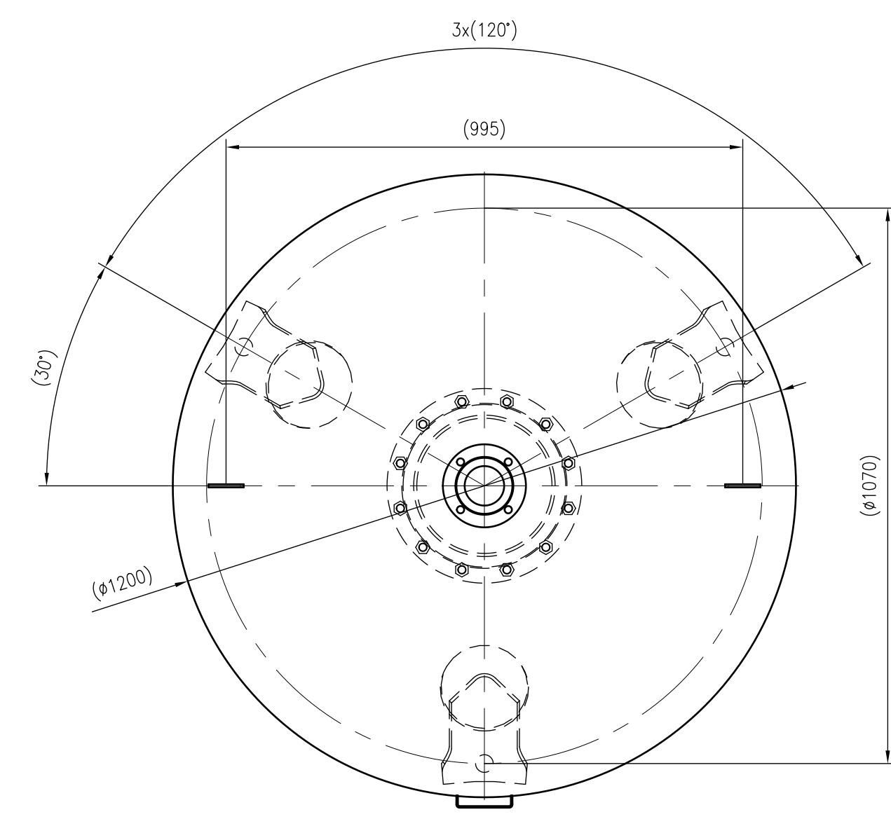
Top view
