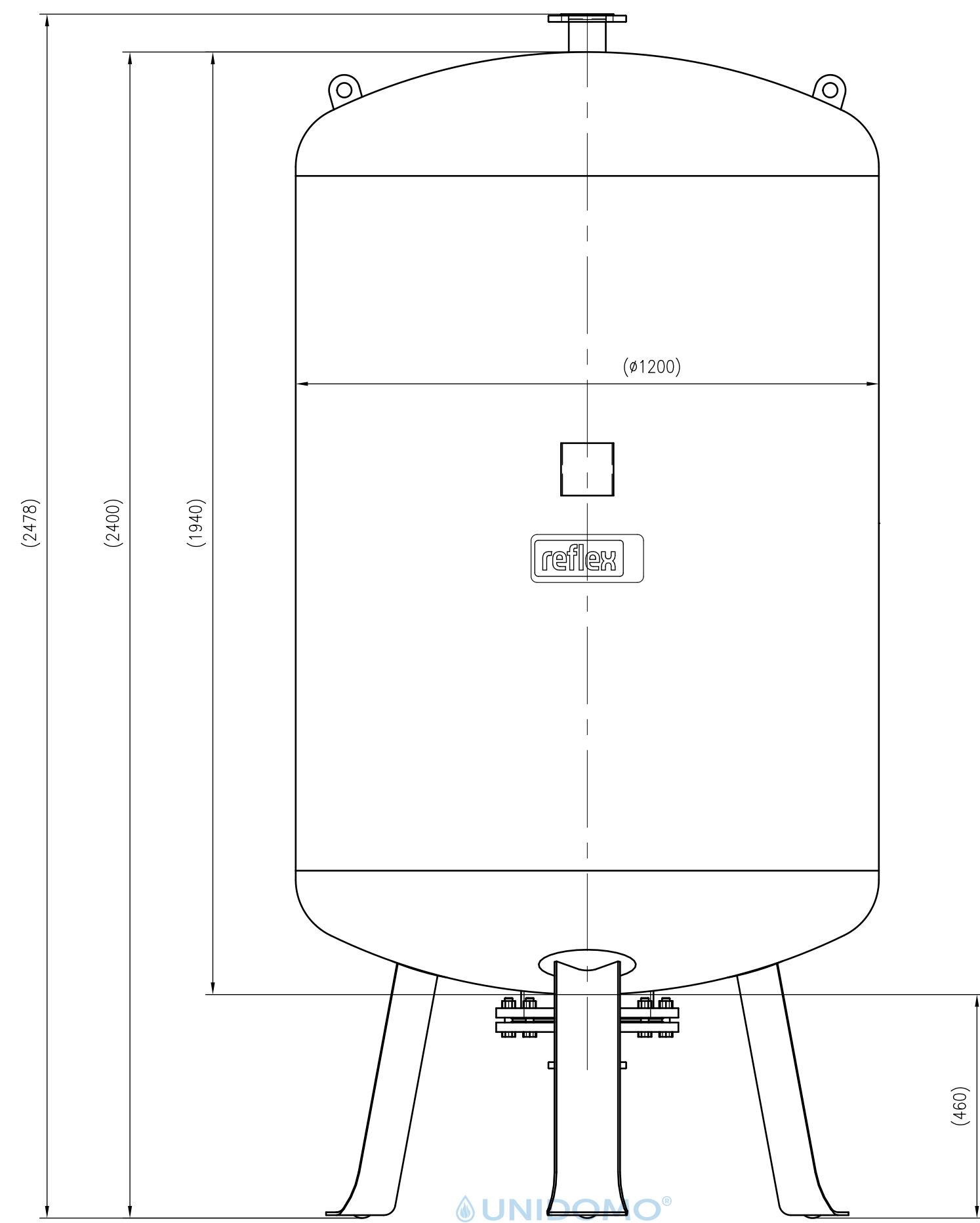
Front view
