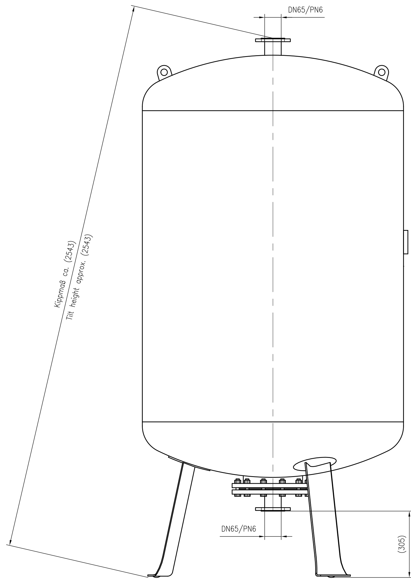
Side view
