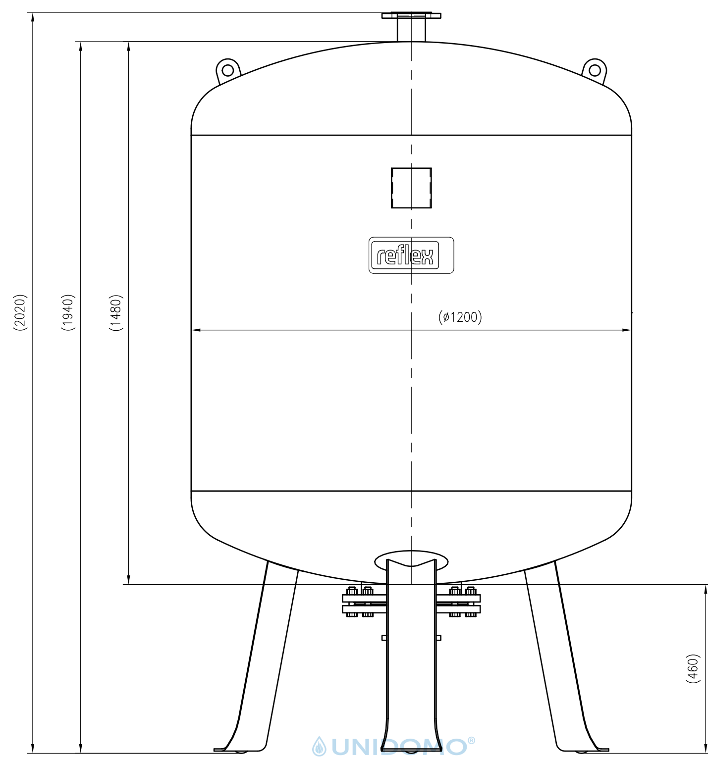
Front view
