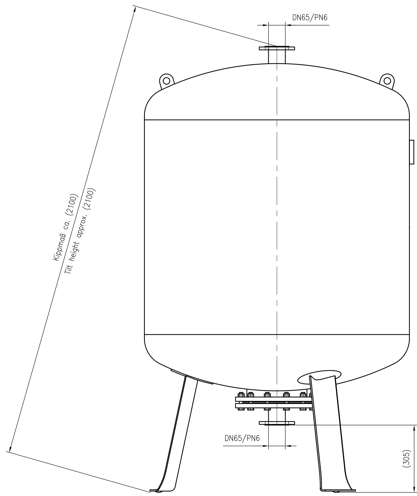
Side view
