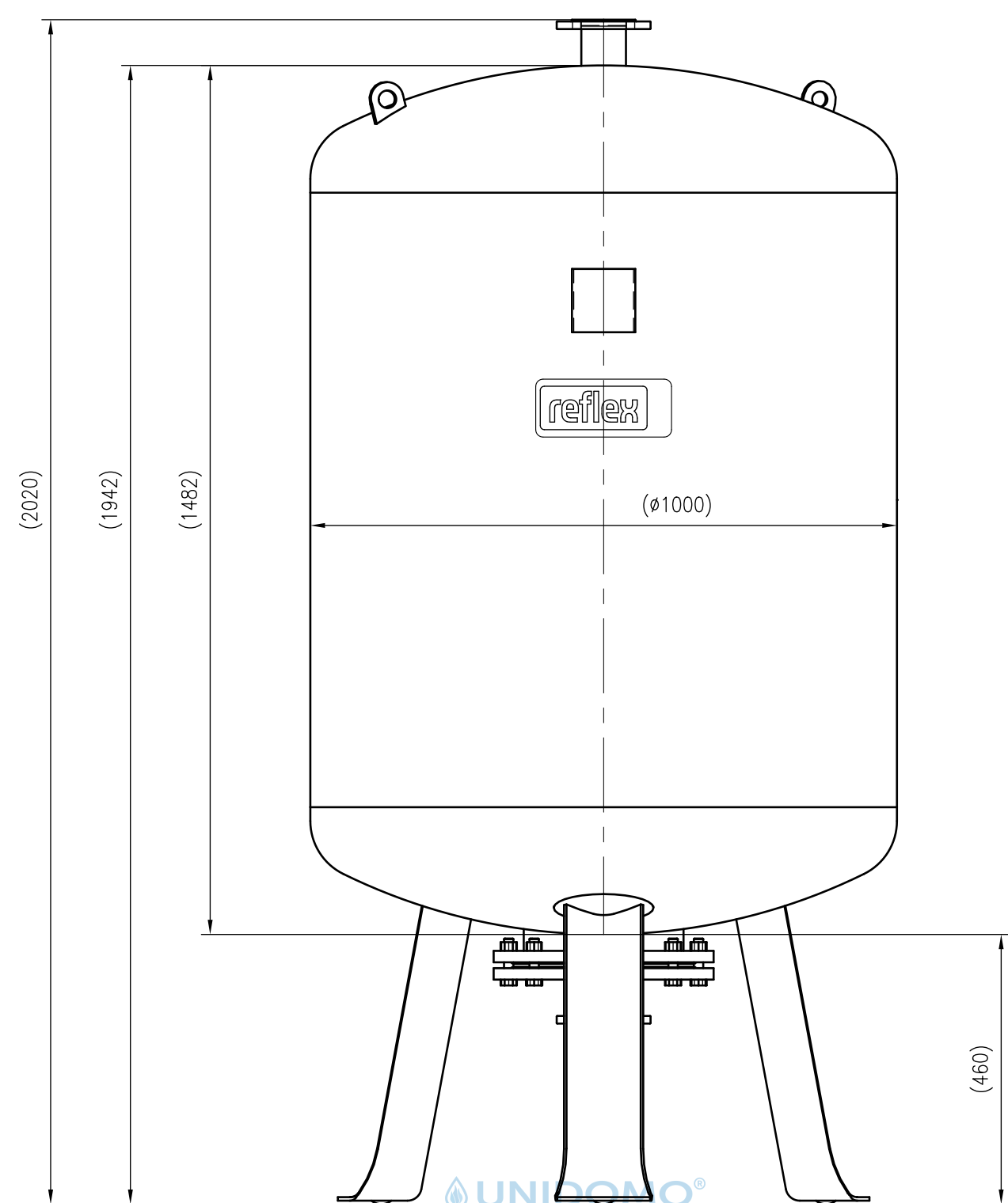
Front view
