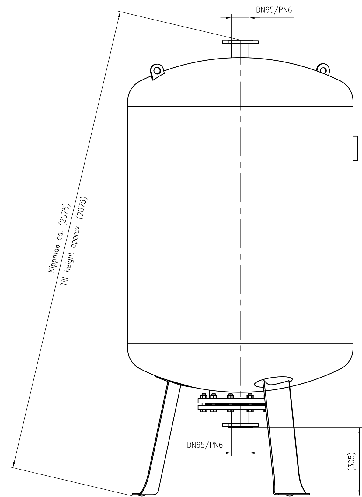
Side view
