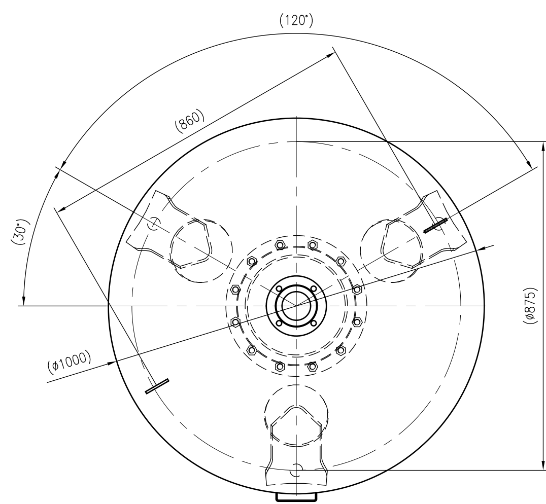
Top view
