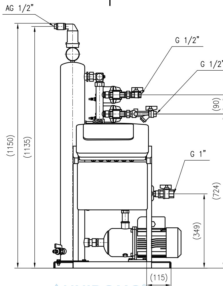
Front view
