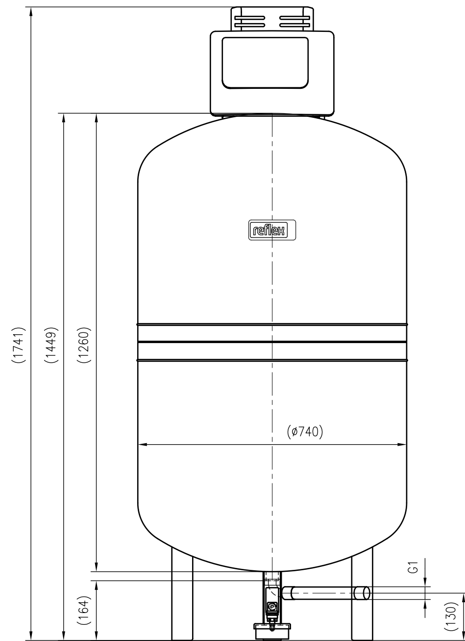
Front view
