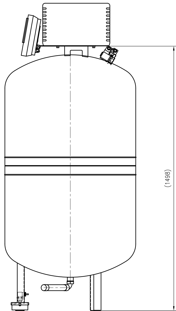
Side view
