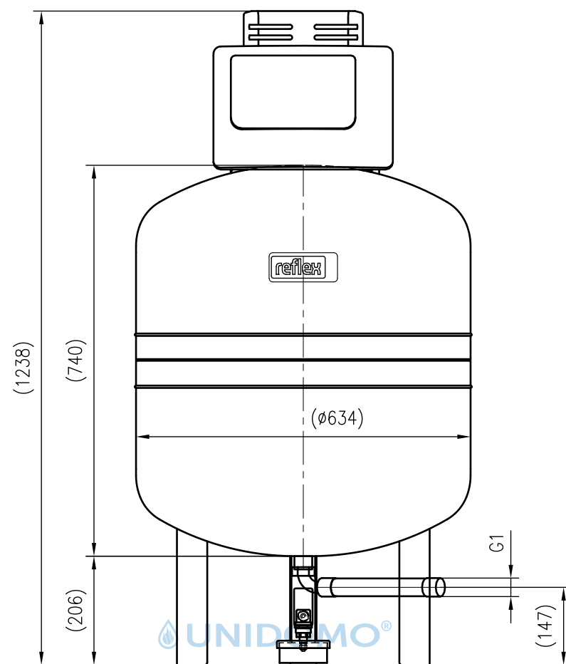
Front view
