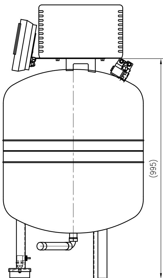
Side view
