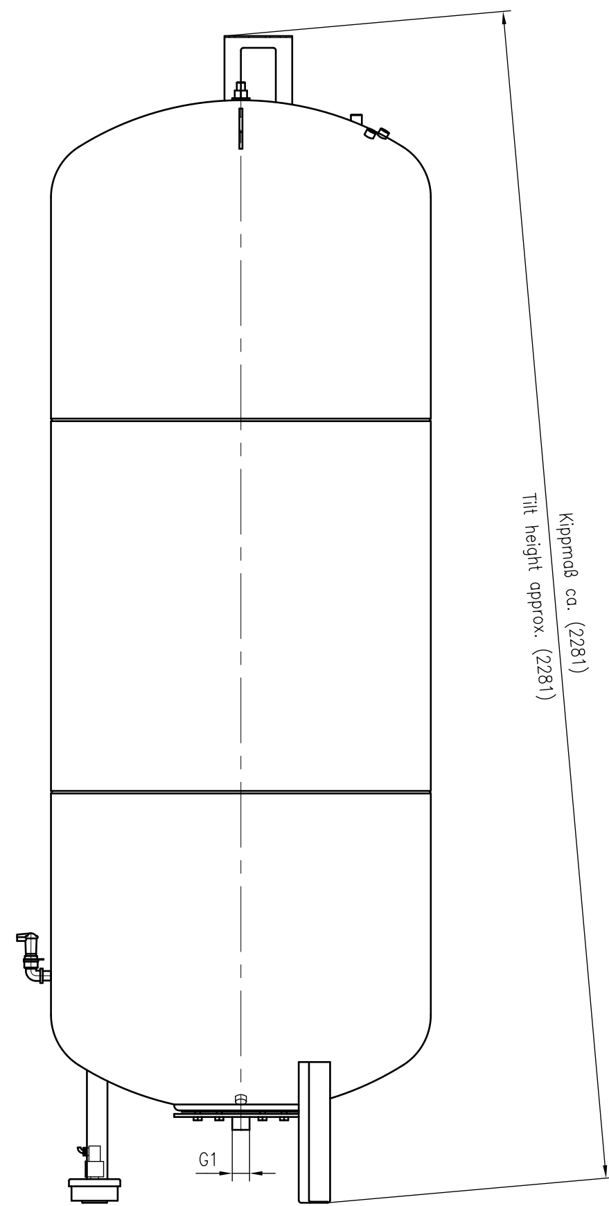
Side view
