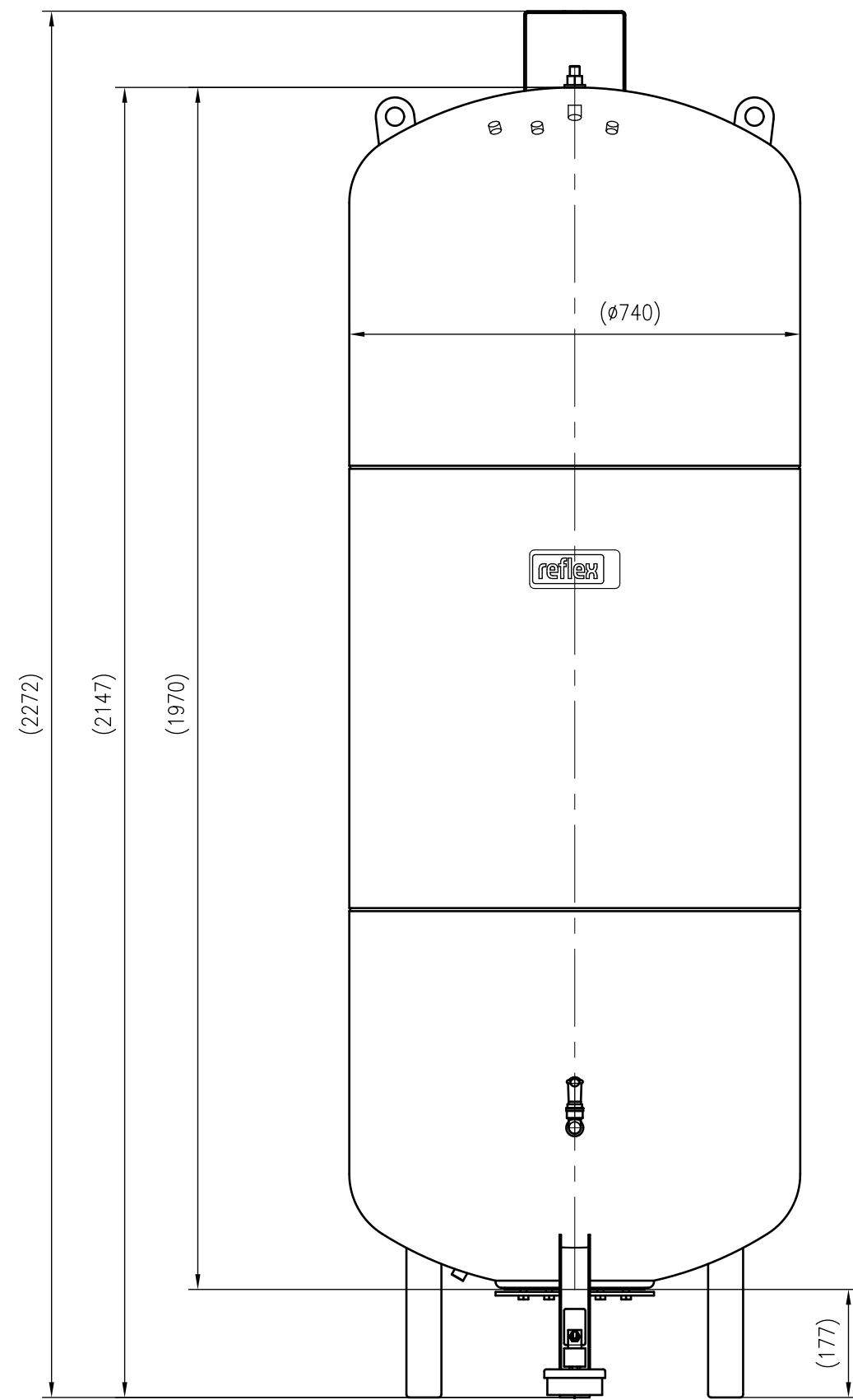
Front view
