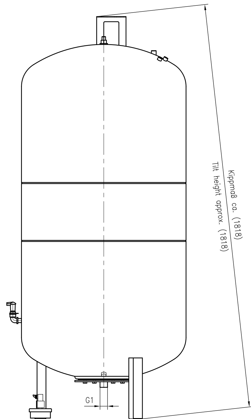
Side view
