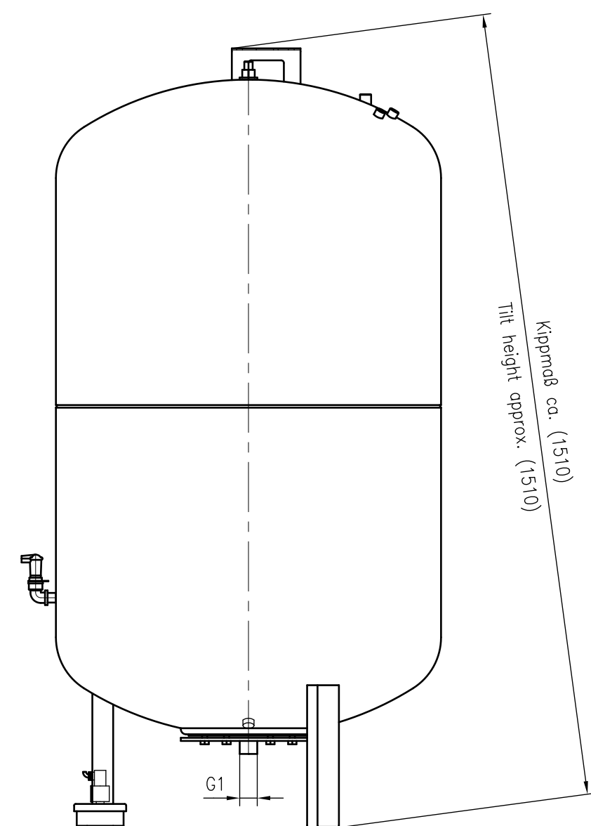
Side view
