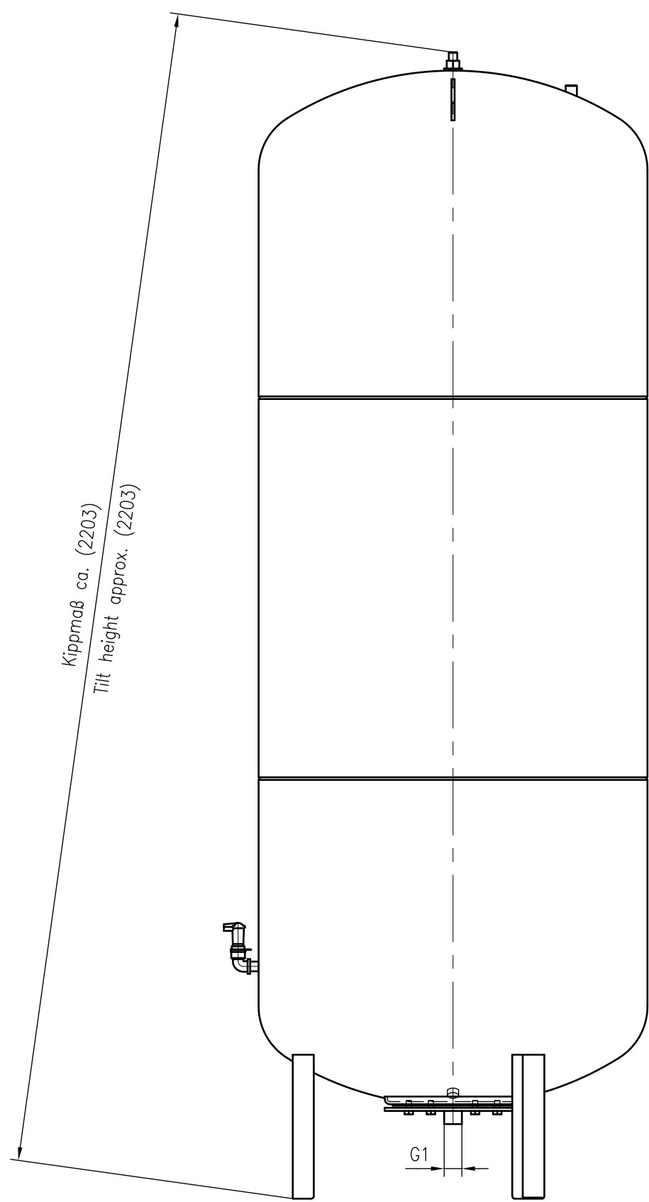
Side view
