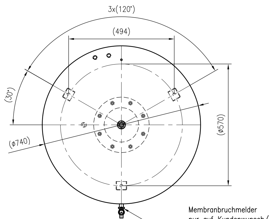
Top view
