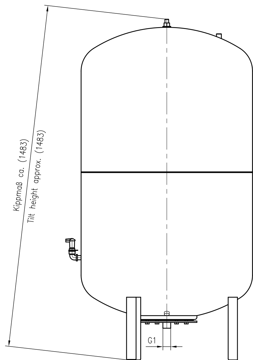
Side view
