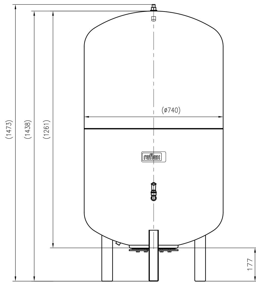
Front view
