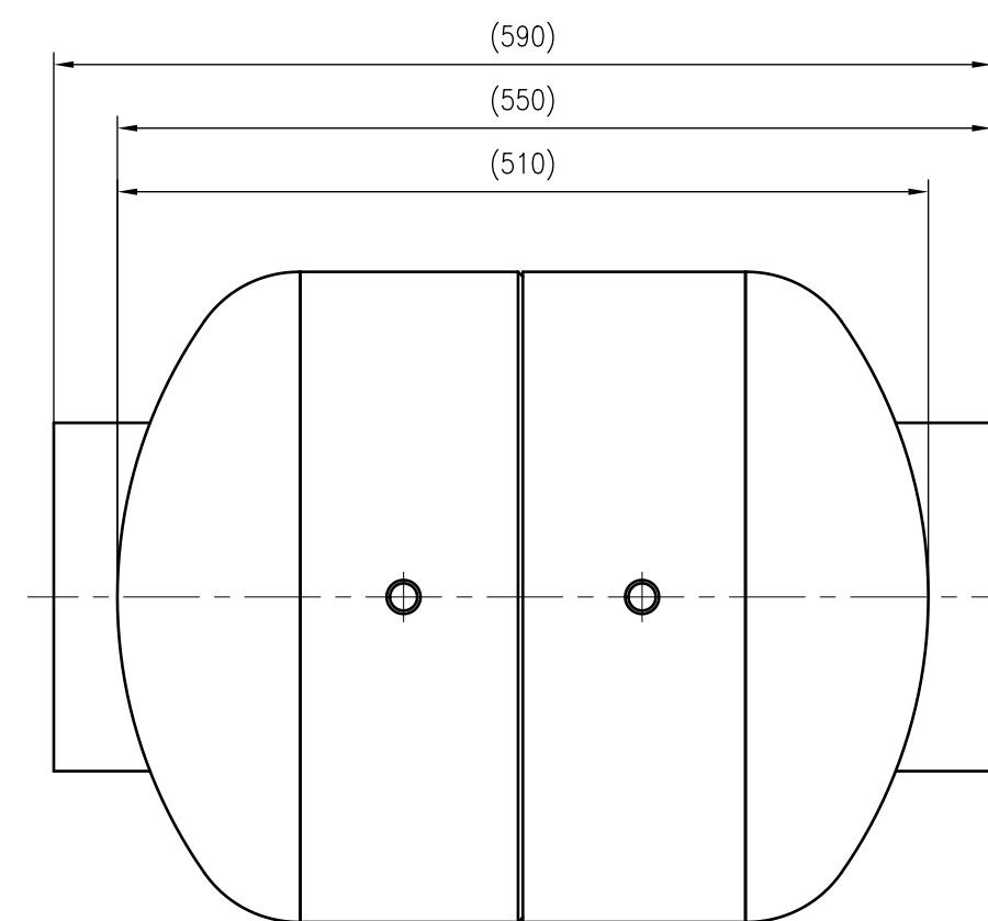
Top view
