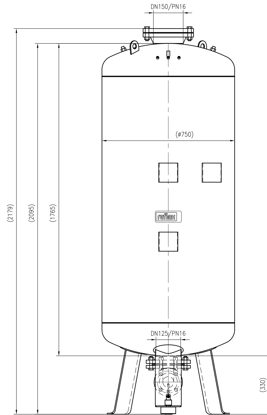
Front view
