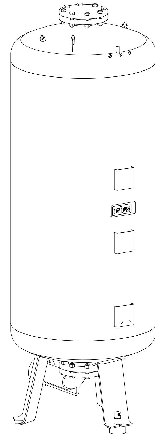
Isometric view
