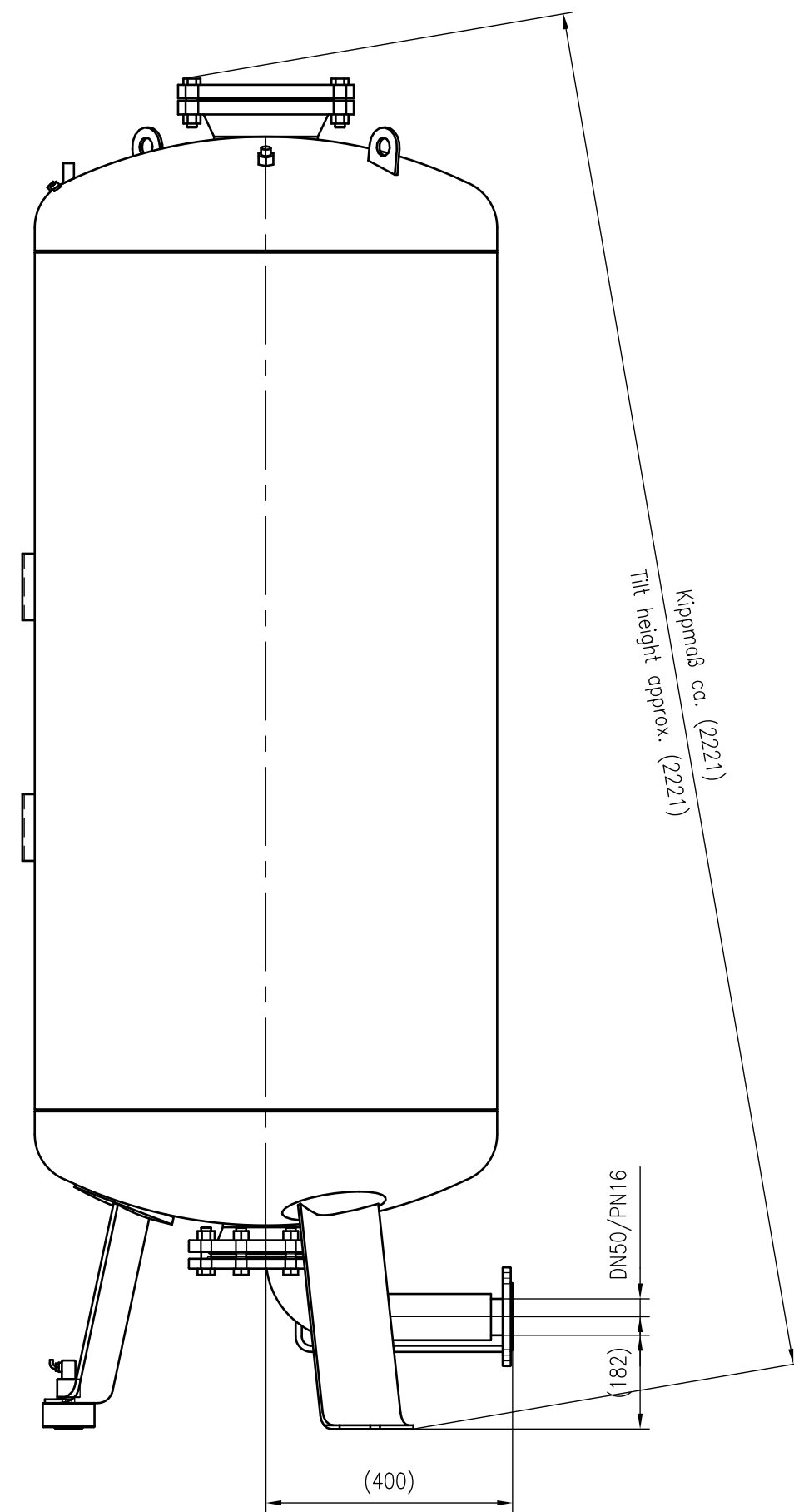
Side view
