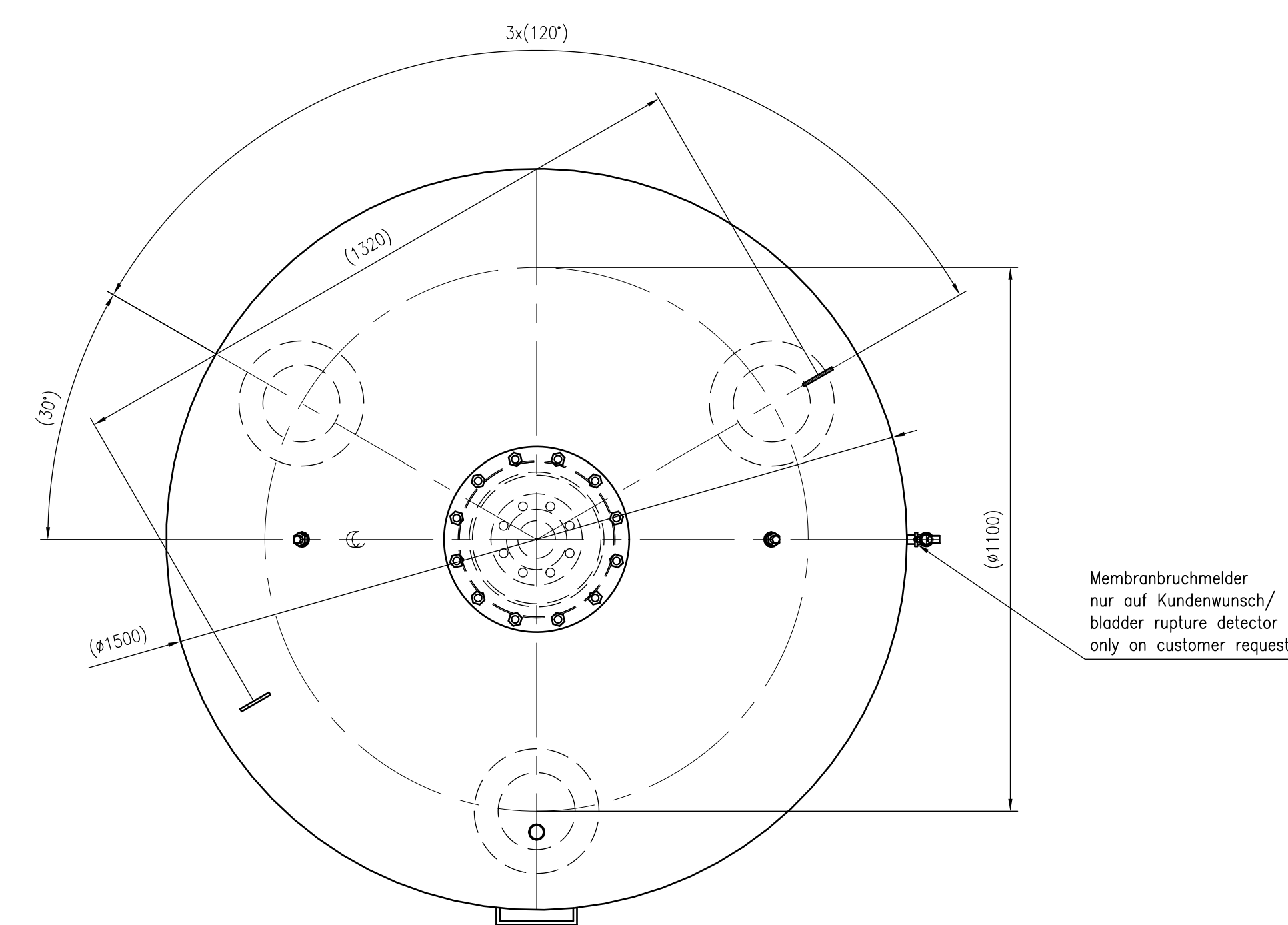
Top view
