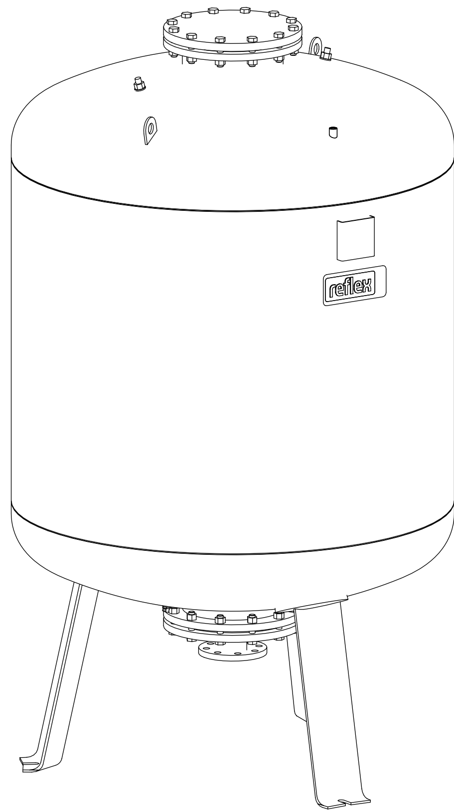
Isometric view
