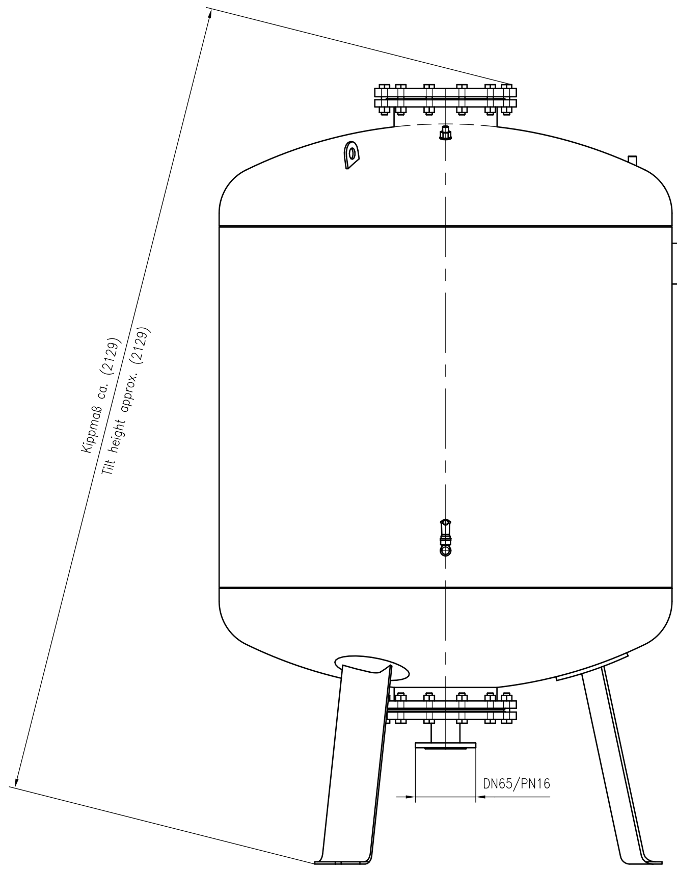
Side view
