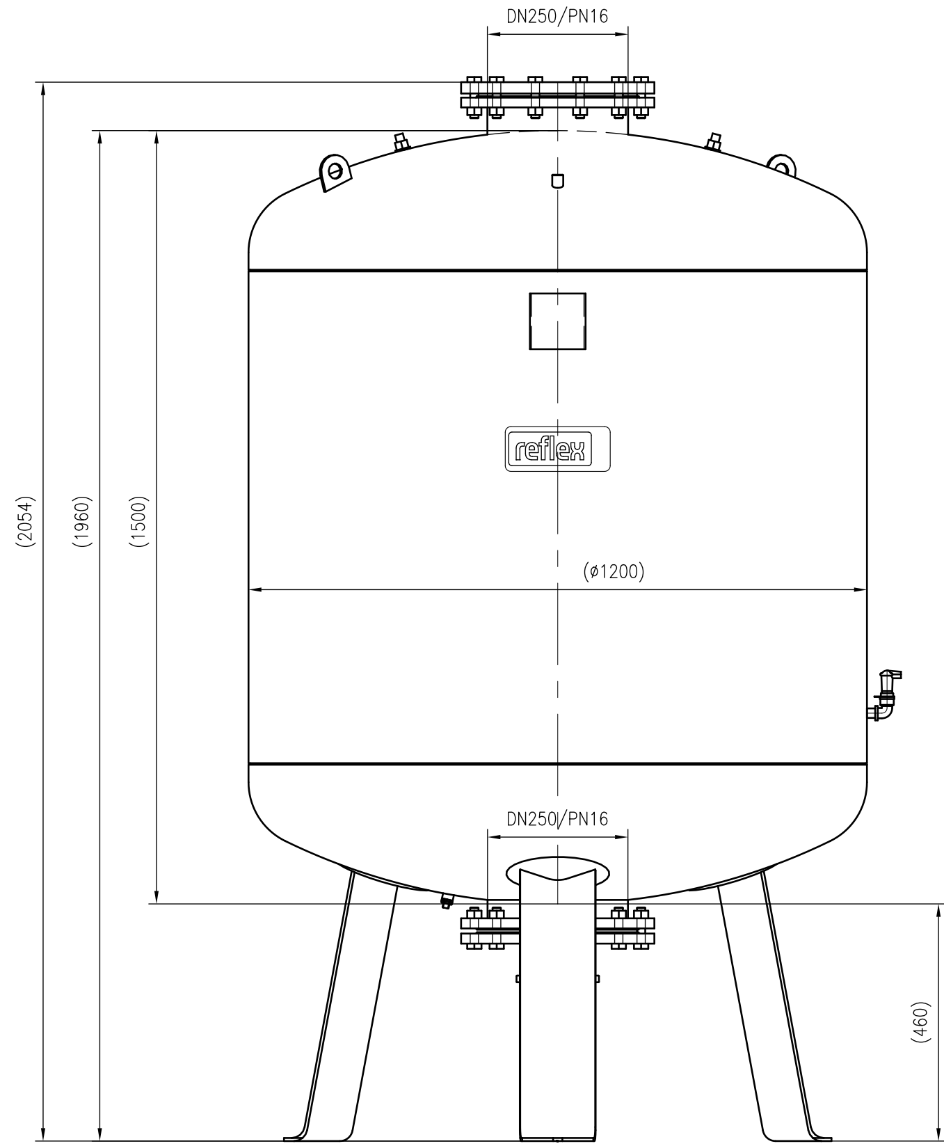
Front view
