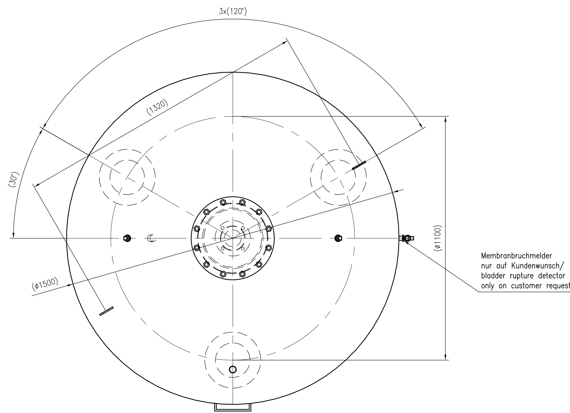
Top view
