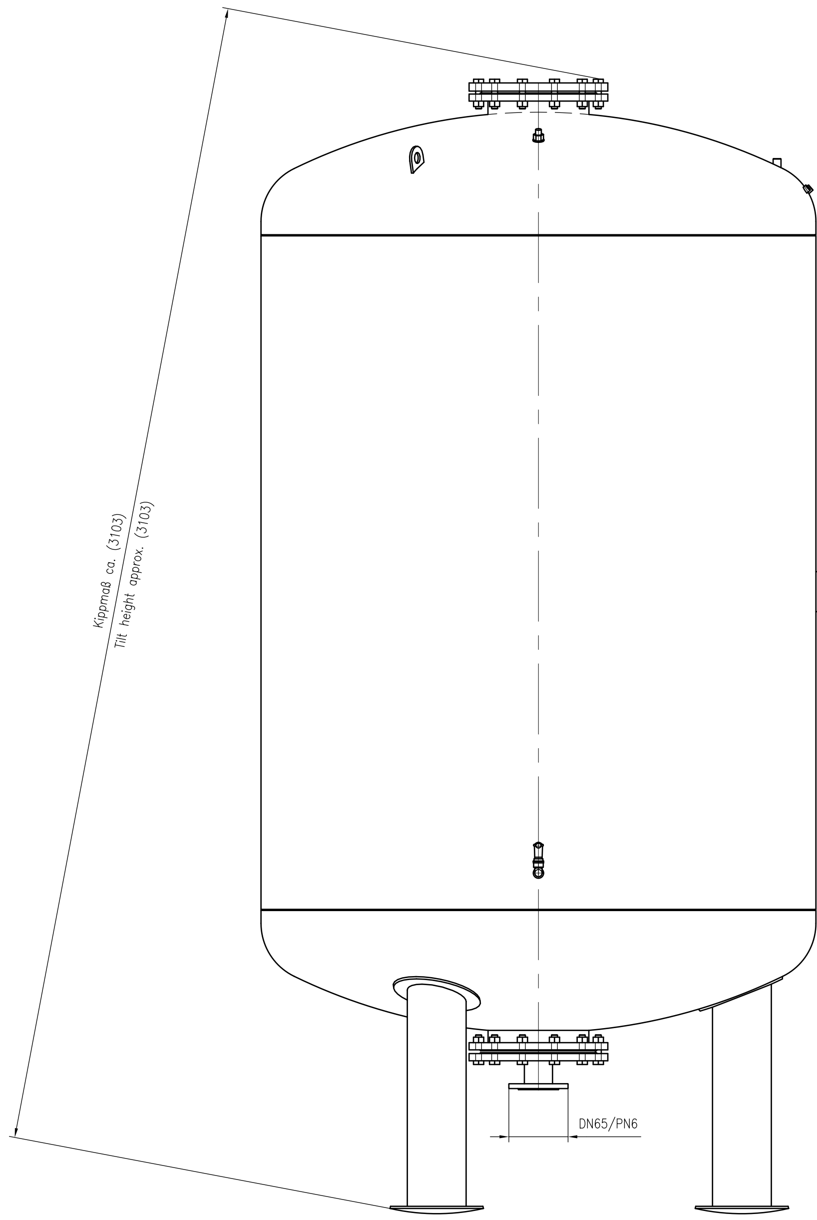
Side view
