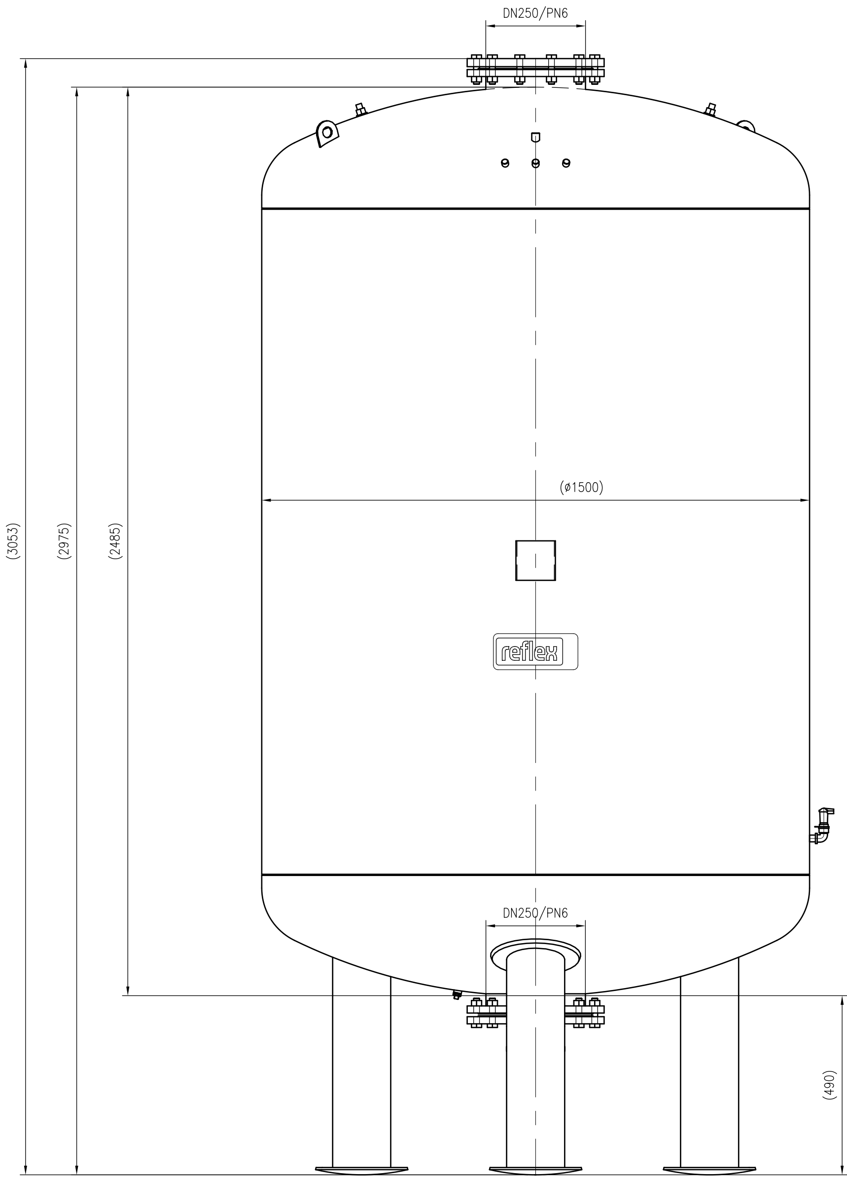
Front view
