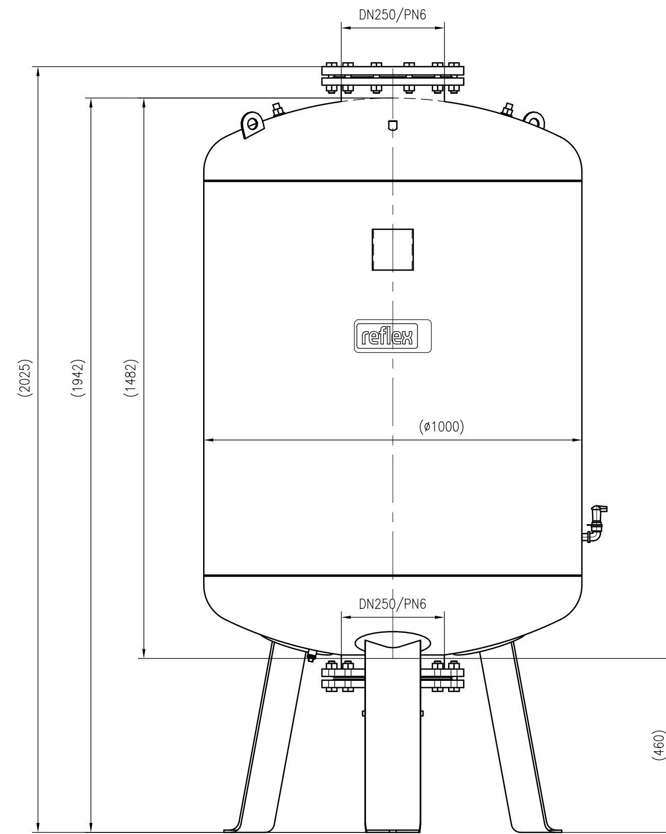
Front view
