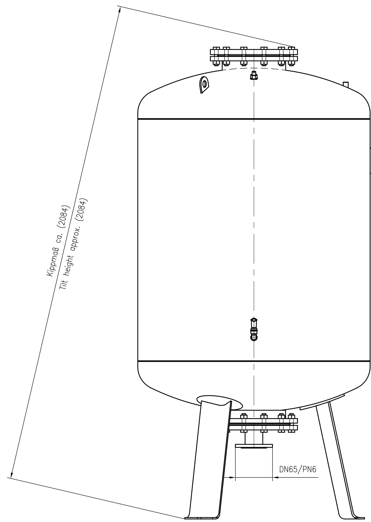
Side view
