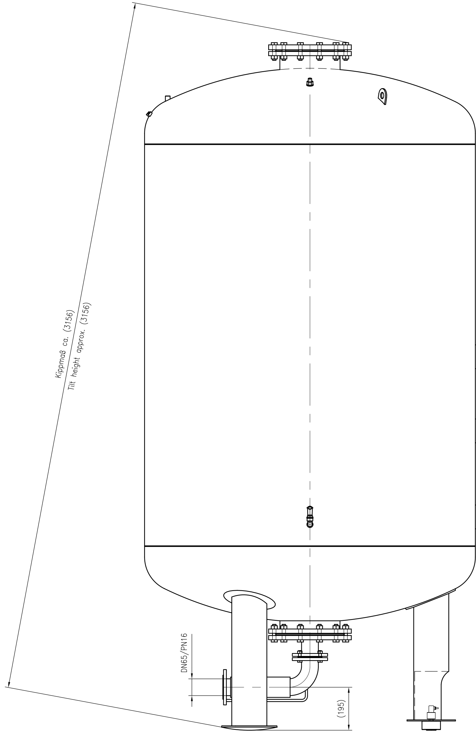
Side view
