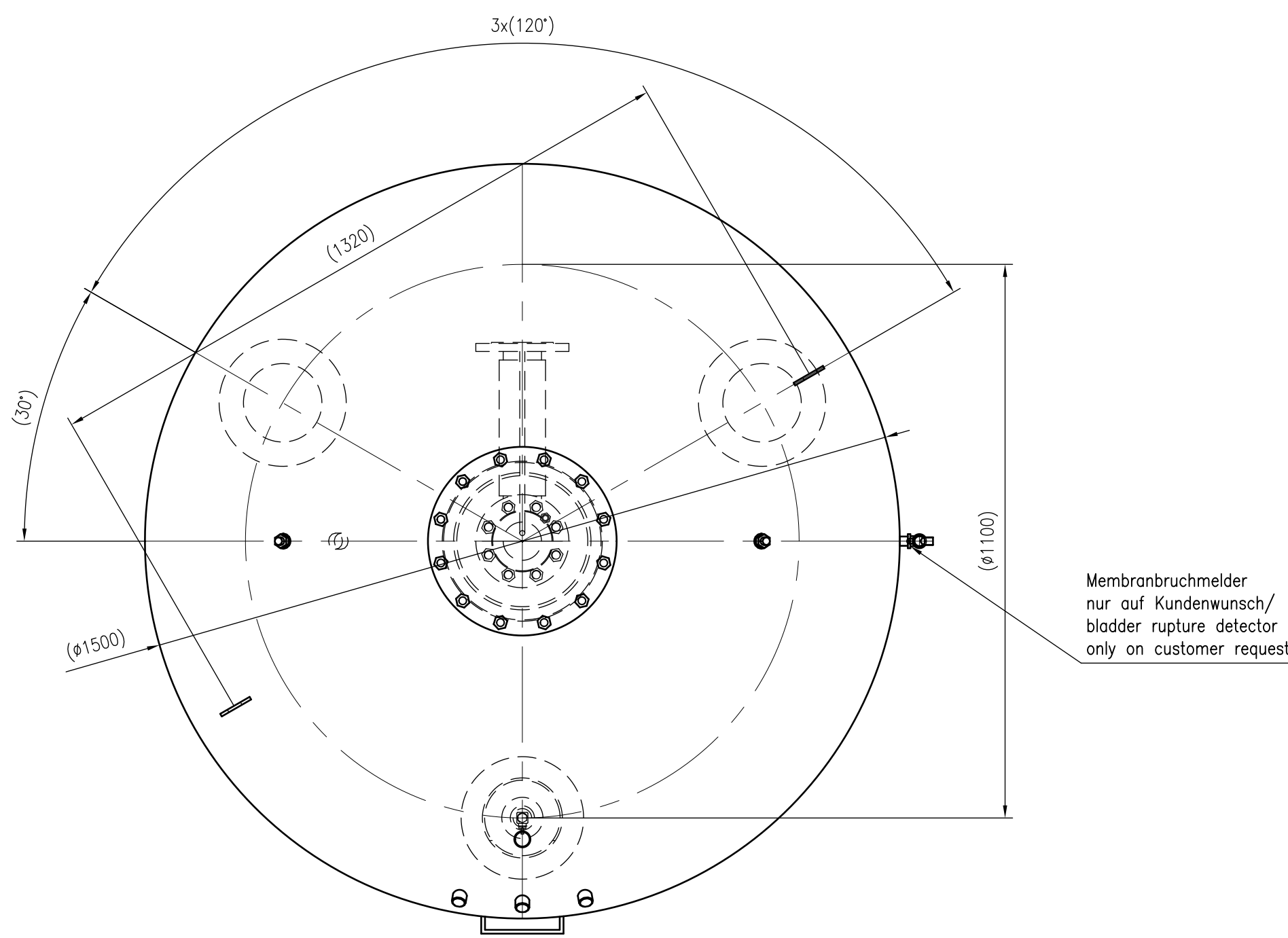
Top view
