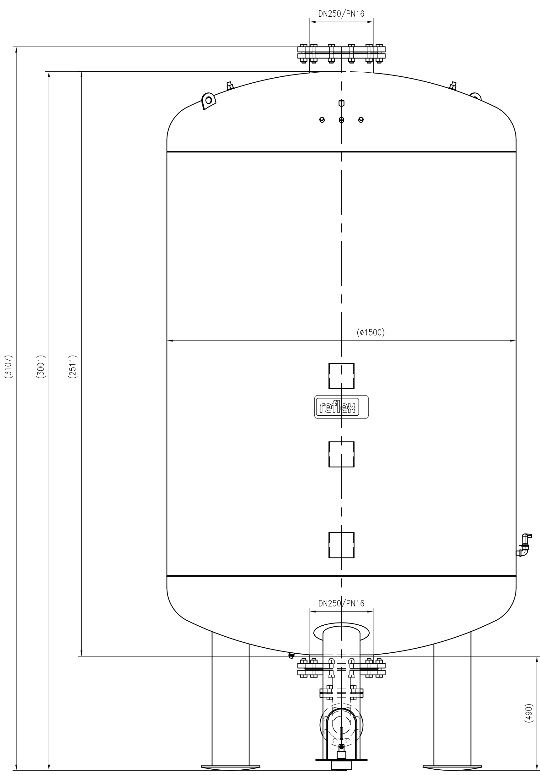
Front view
