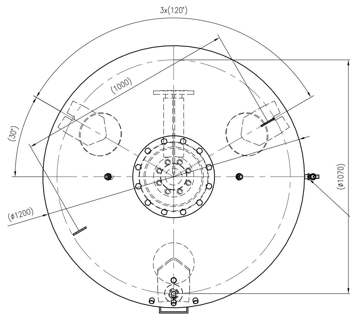
Top view
