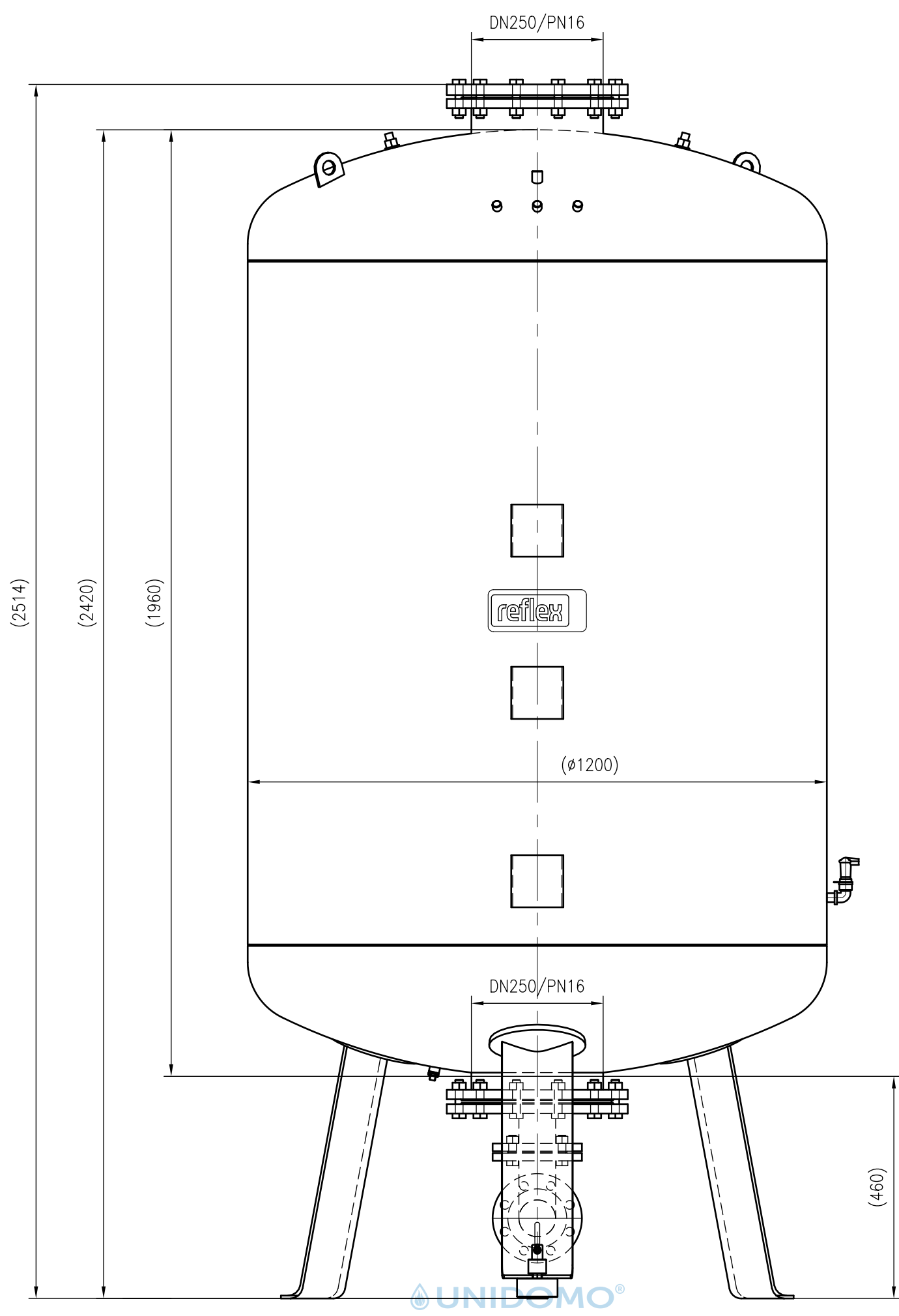
Front view
