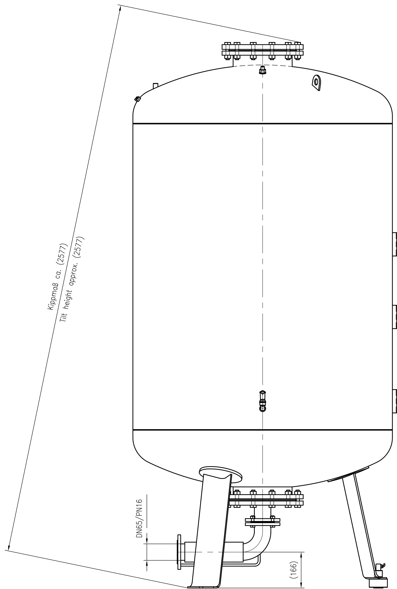
Side view
