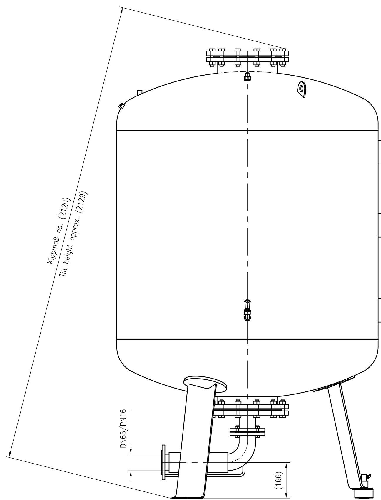
Side view
