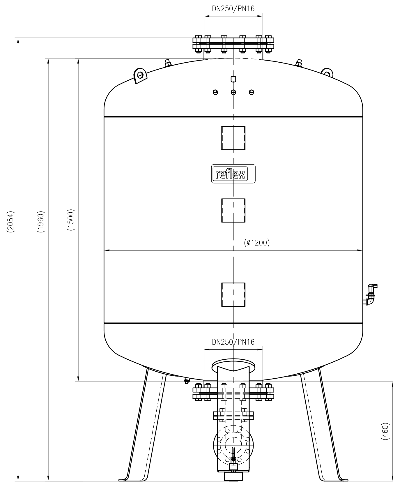
Front view
