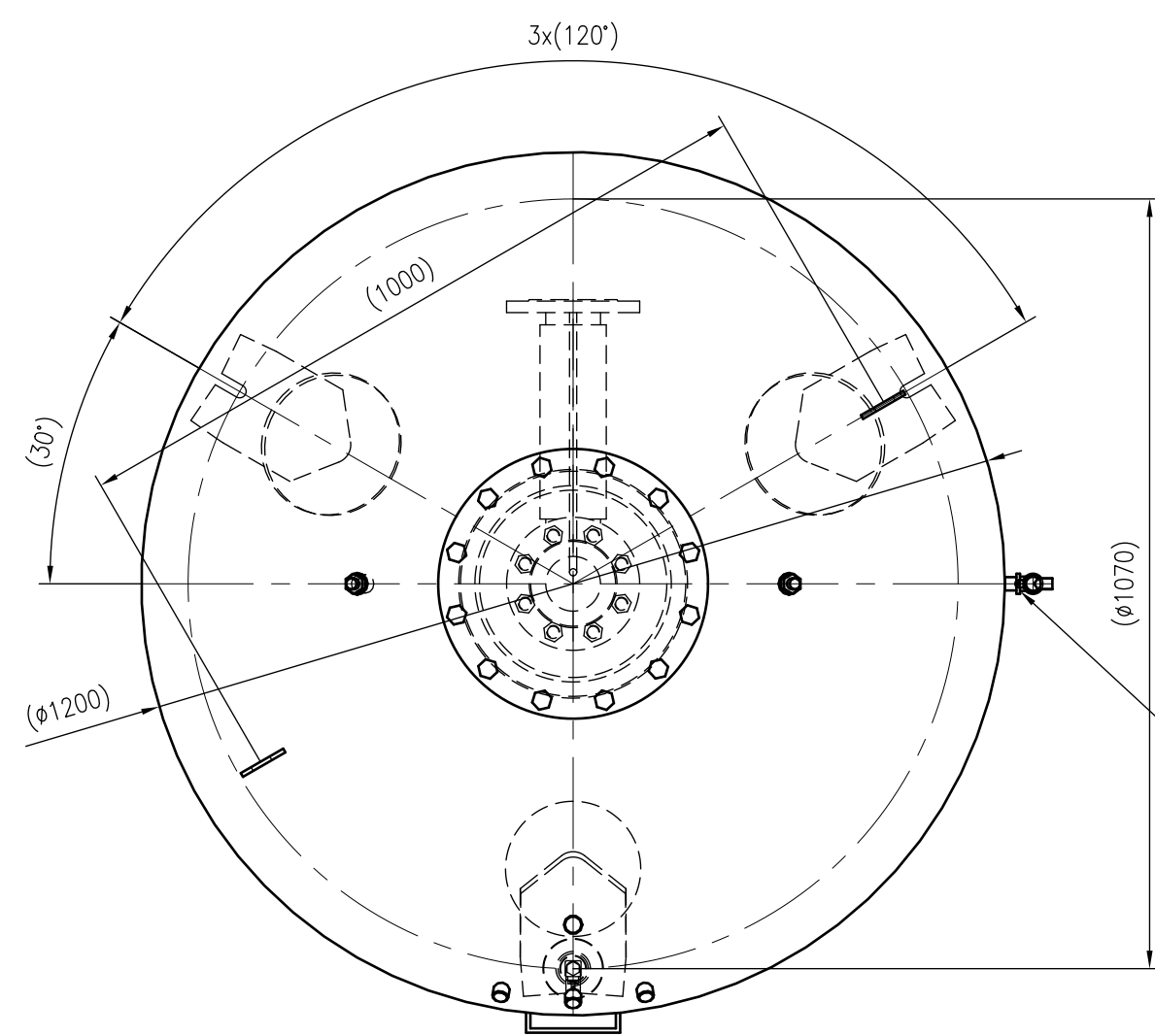
Top view
