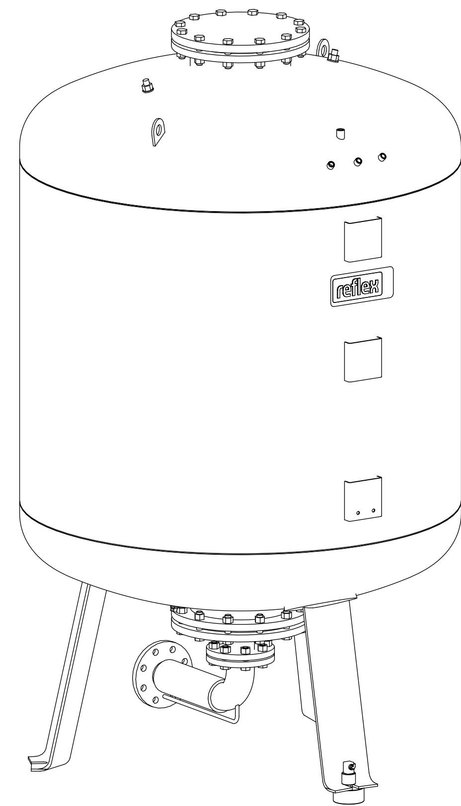
Isometric view
