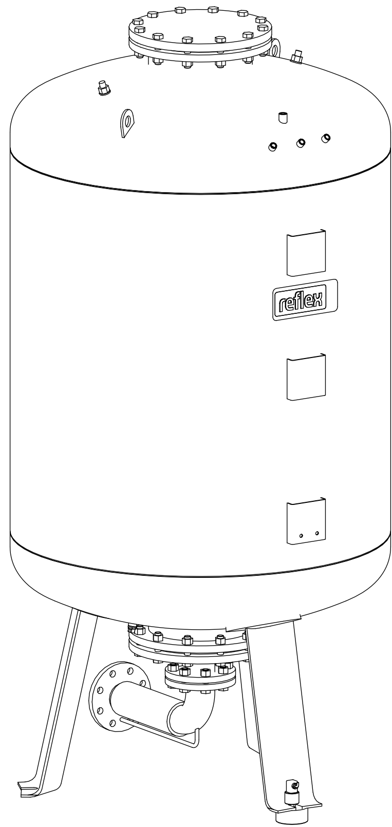
Isometric view
