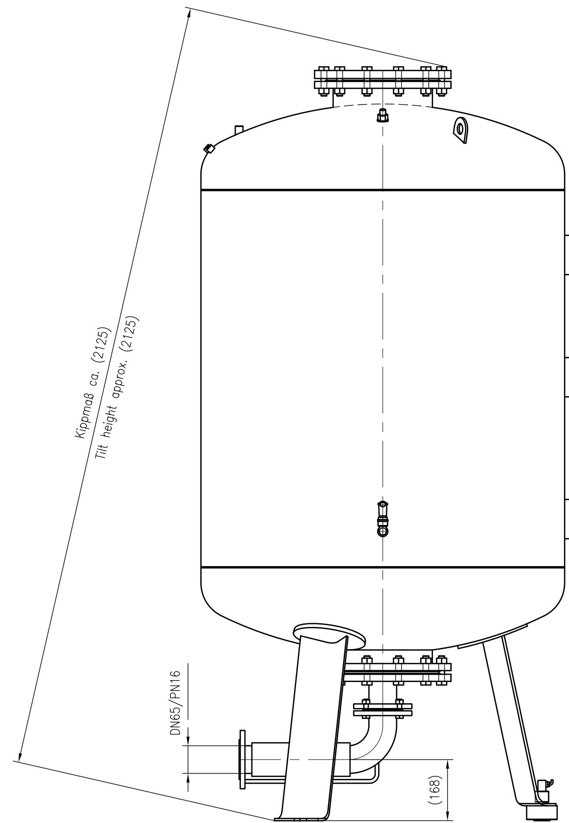
Side view
