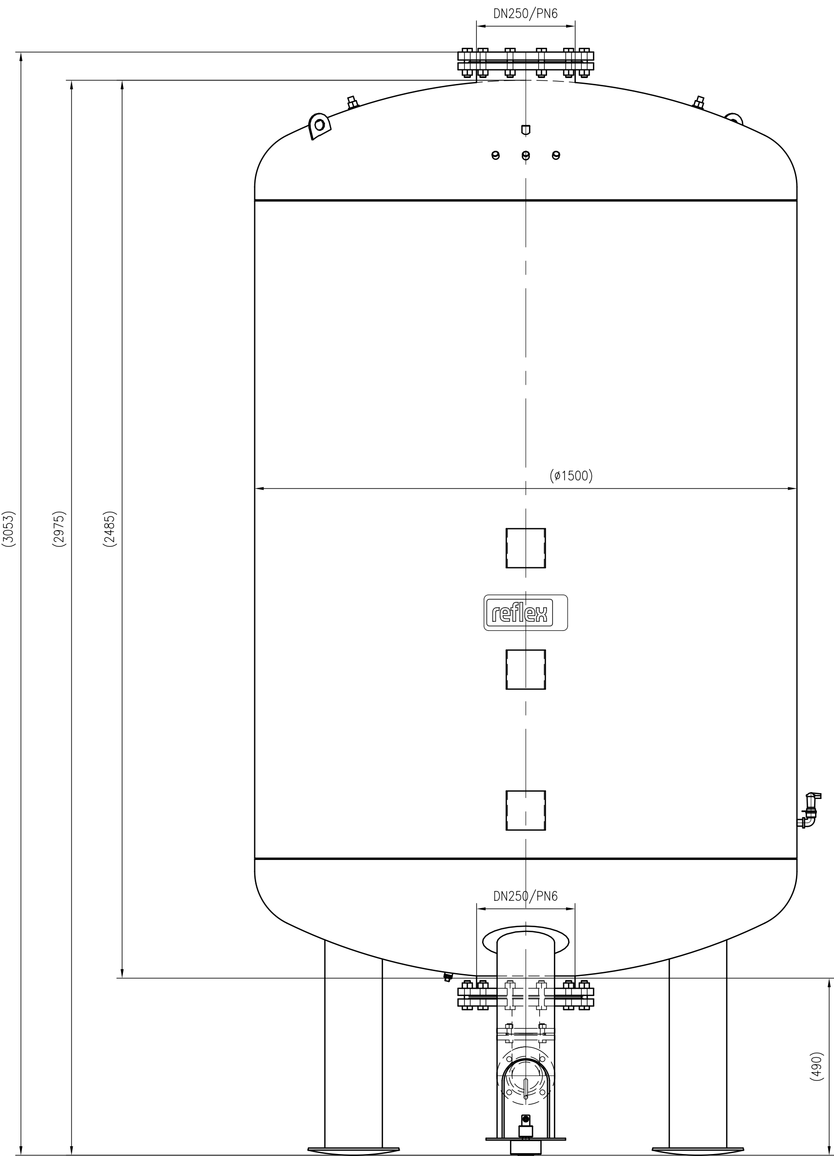
Front view
