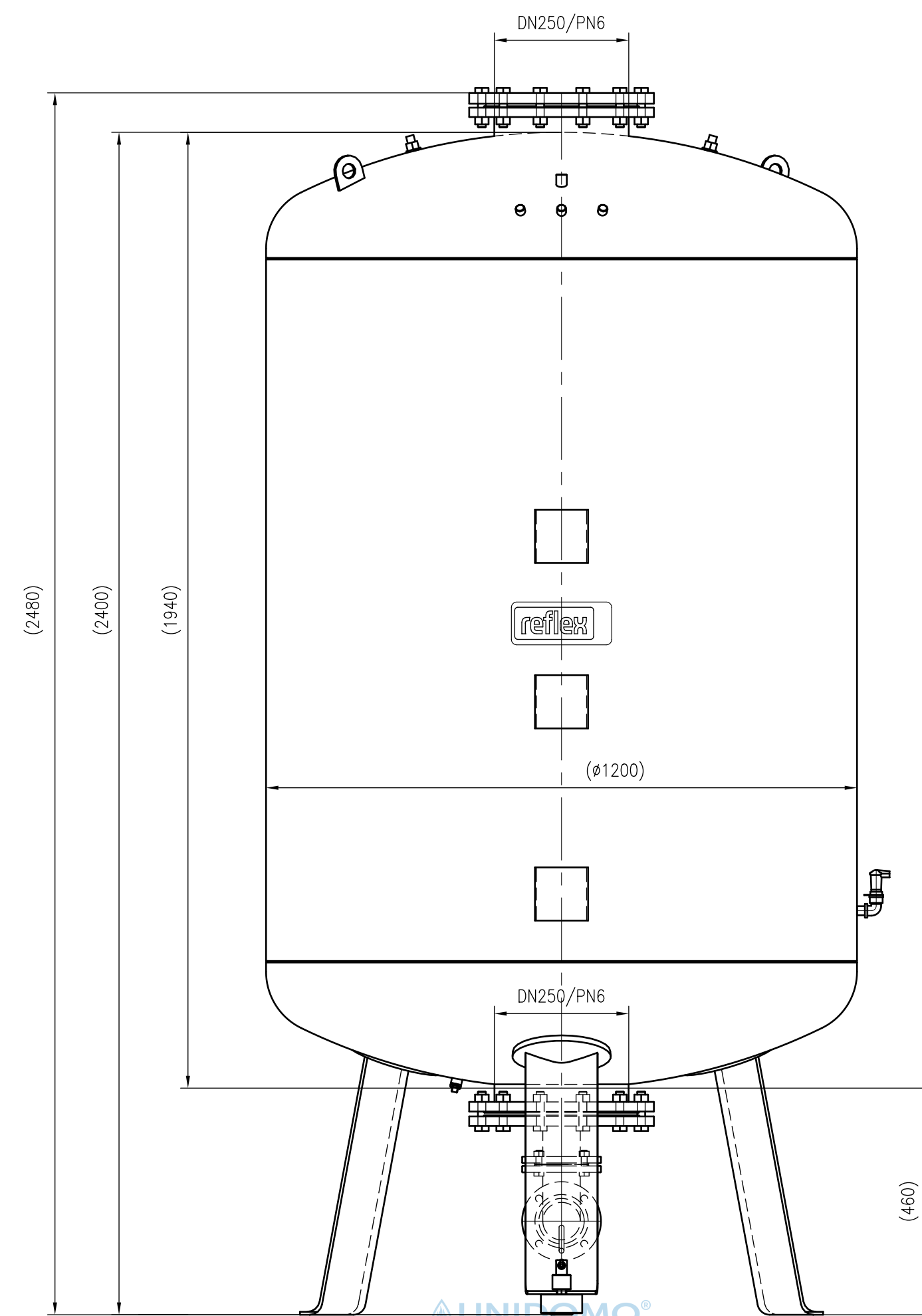
Front view
