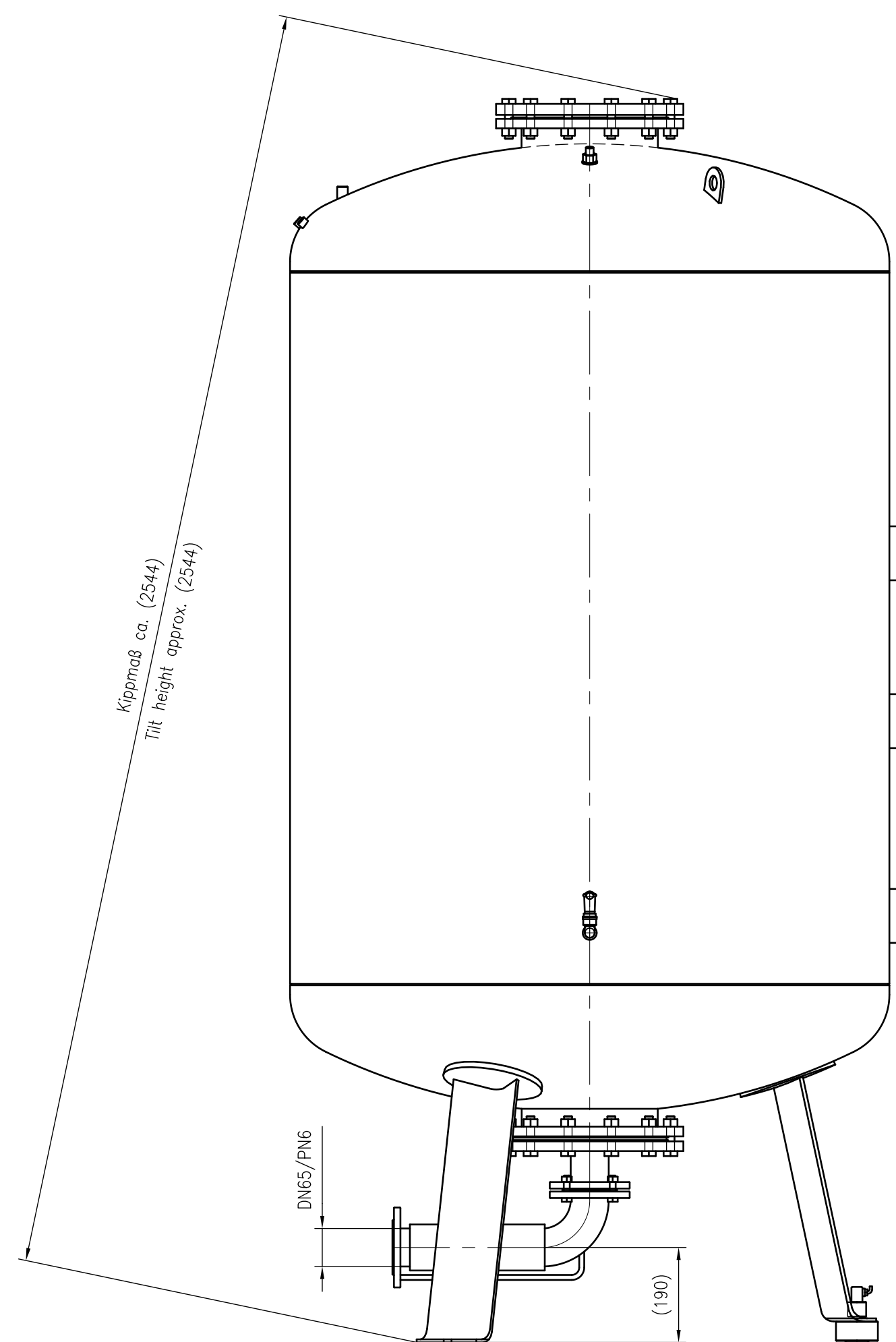
Side view
