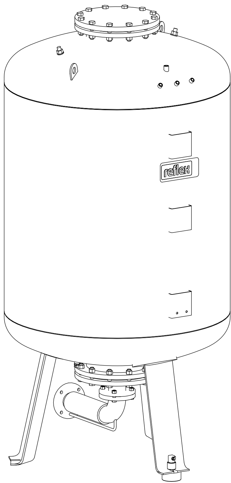
Isometric view
