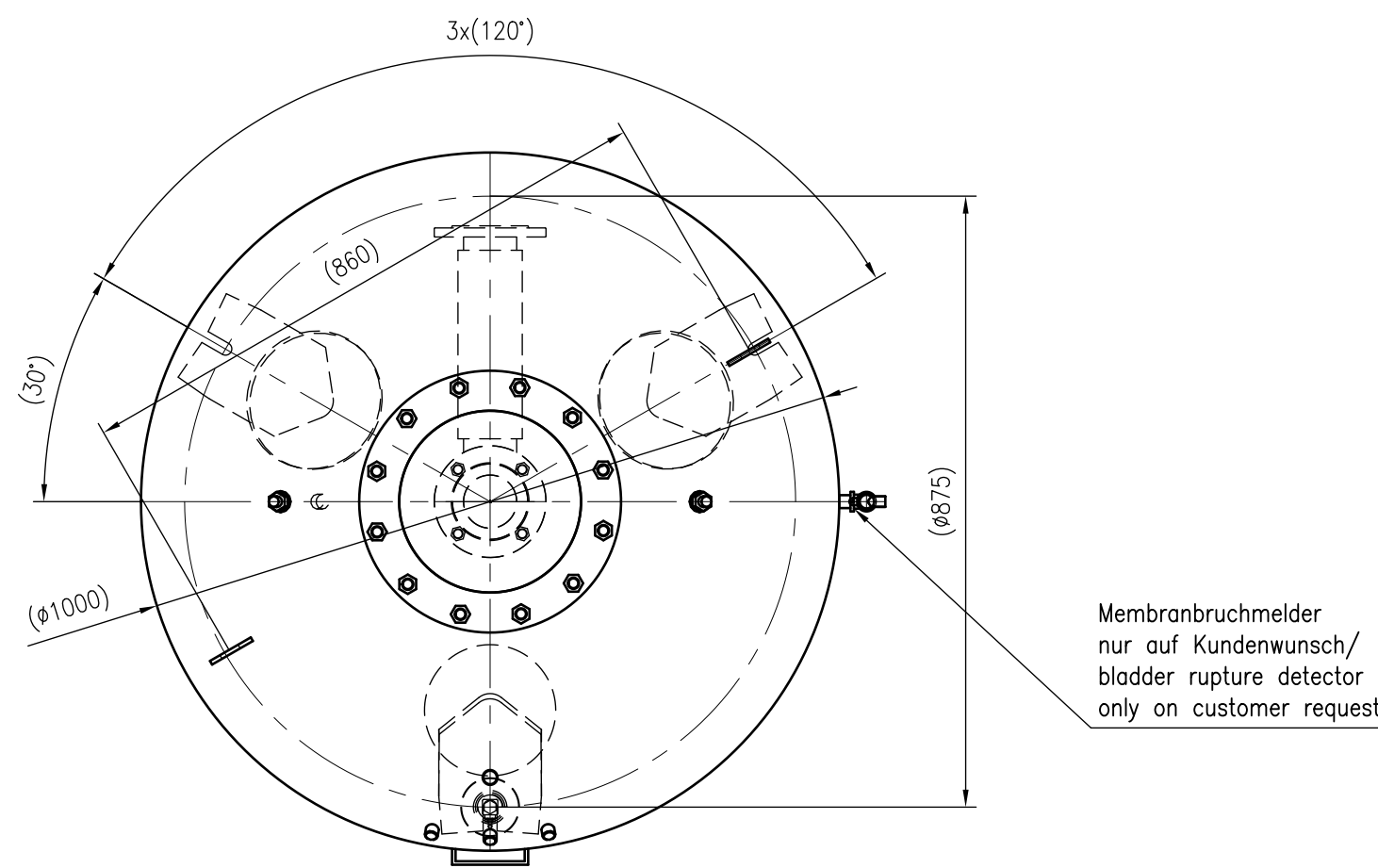
Top view
