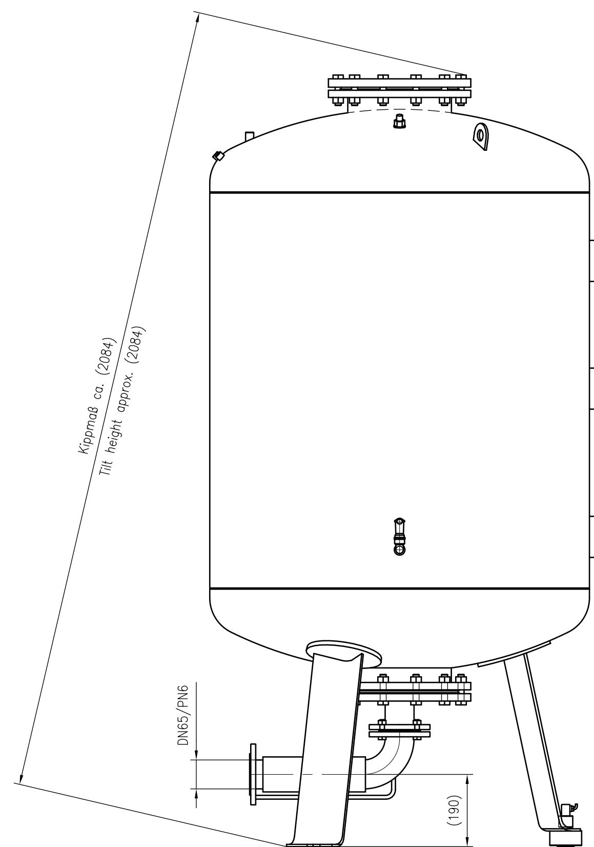
Side view
