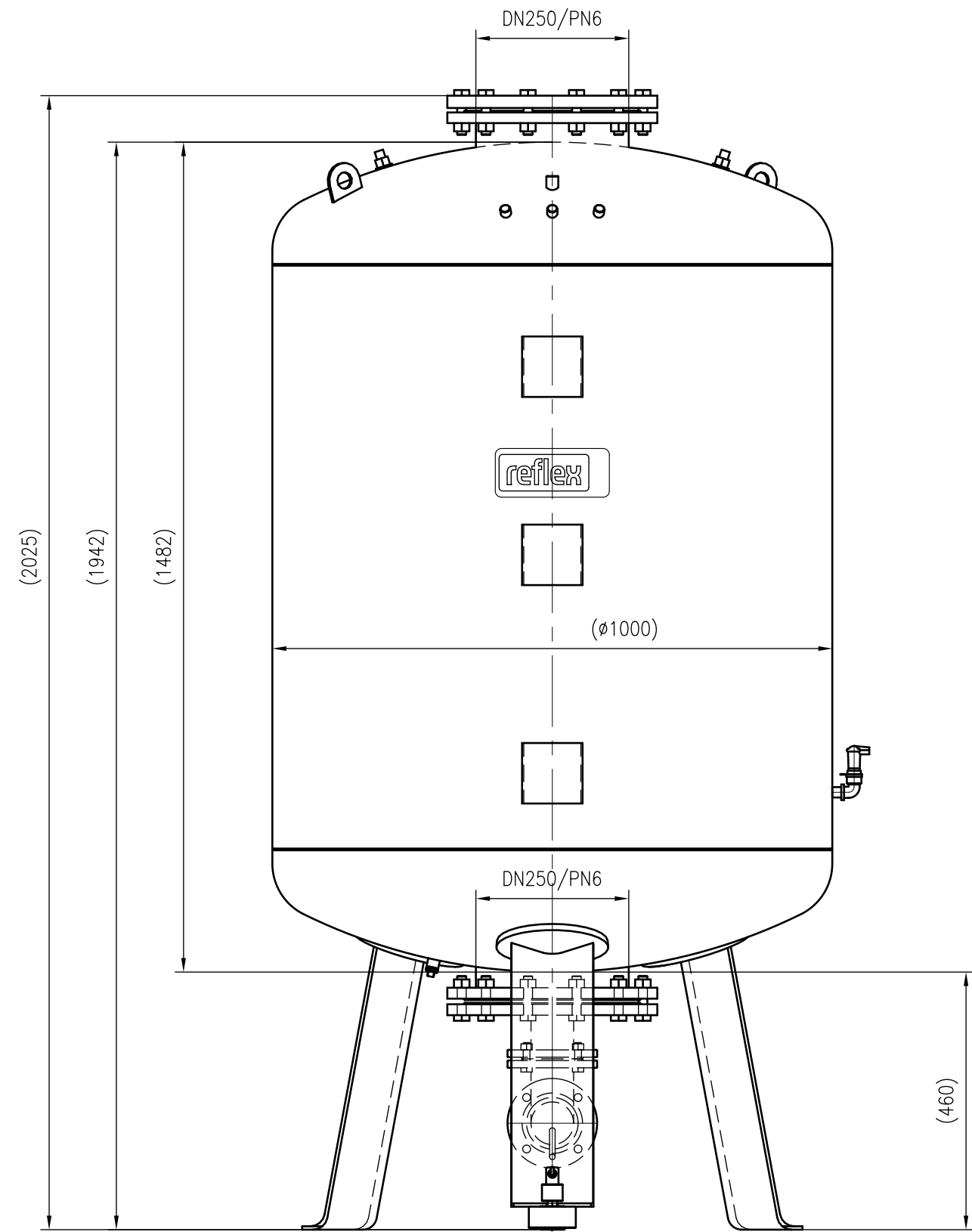
Front view
