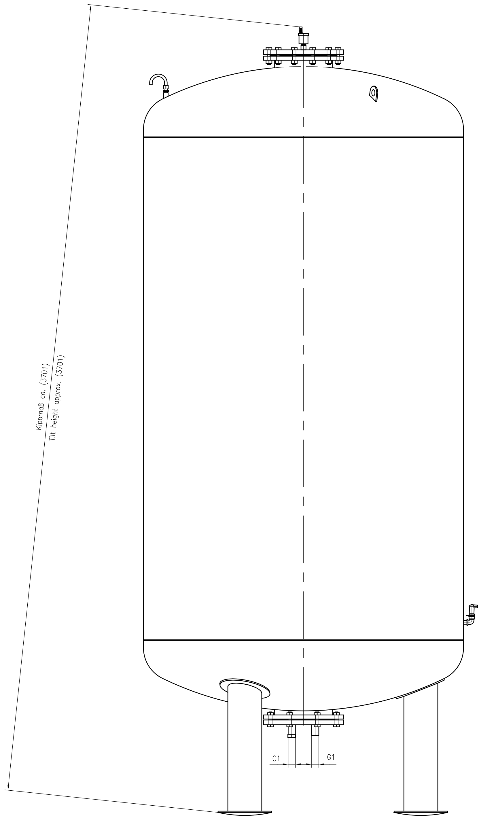
Side view
