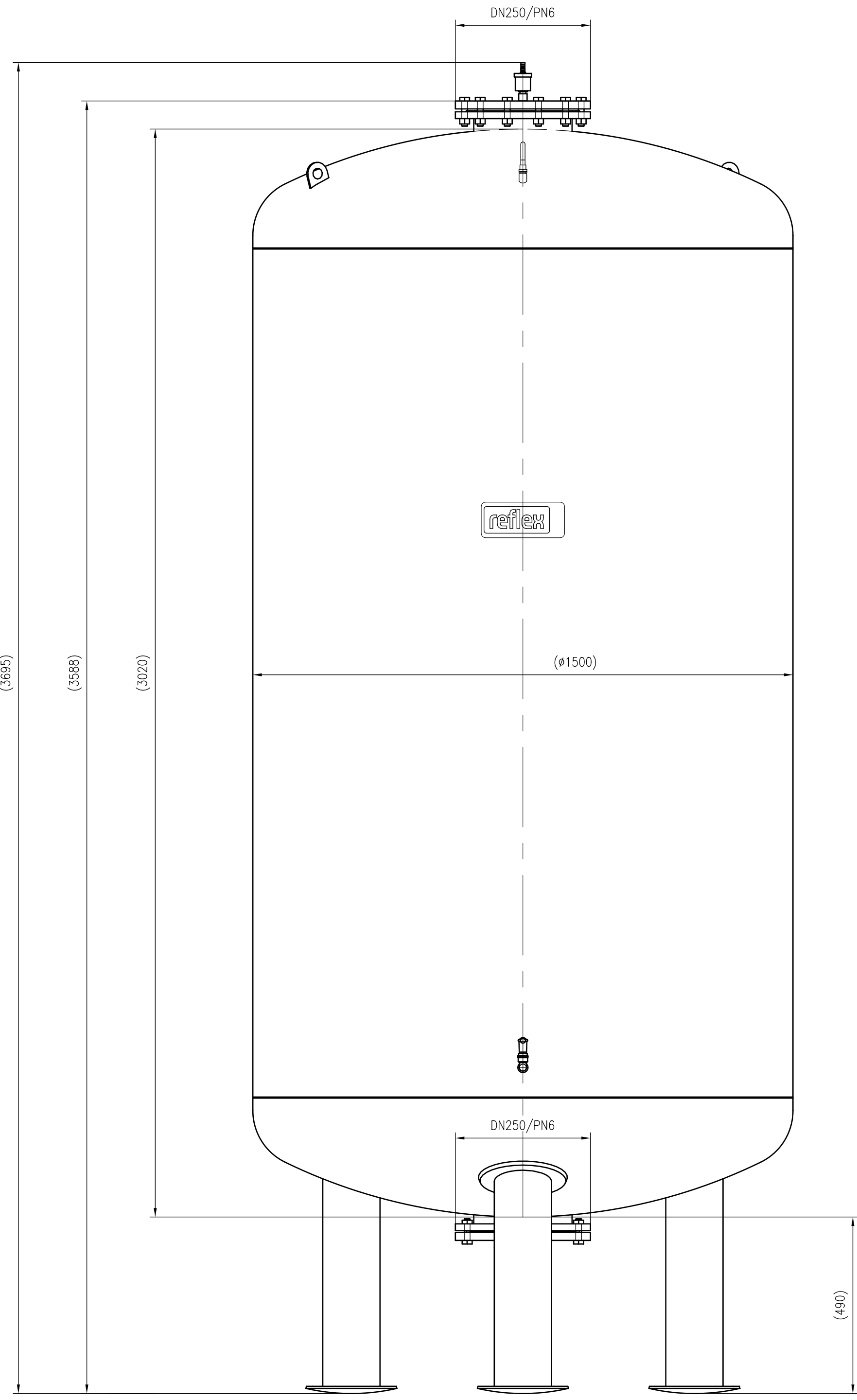
Front view
