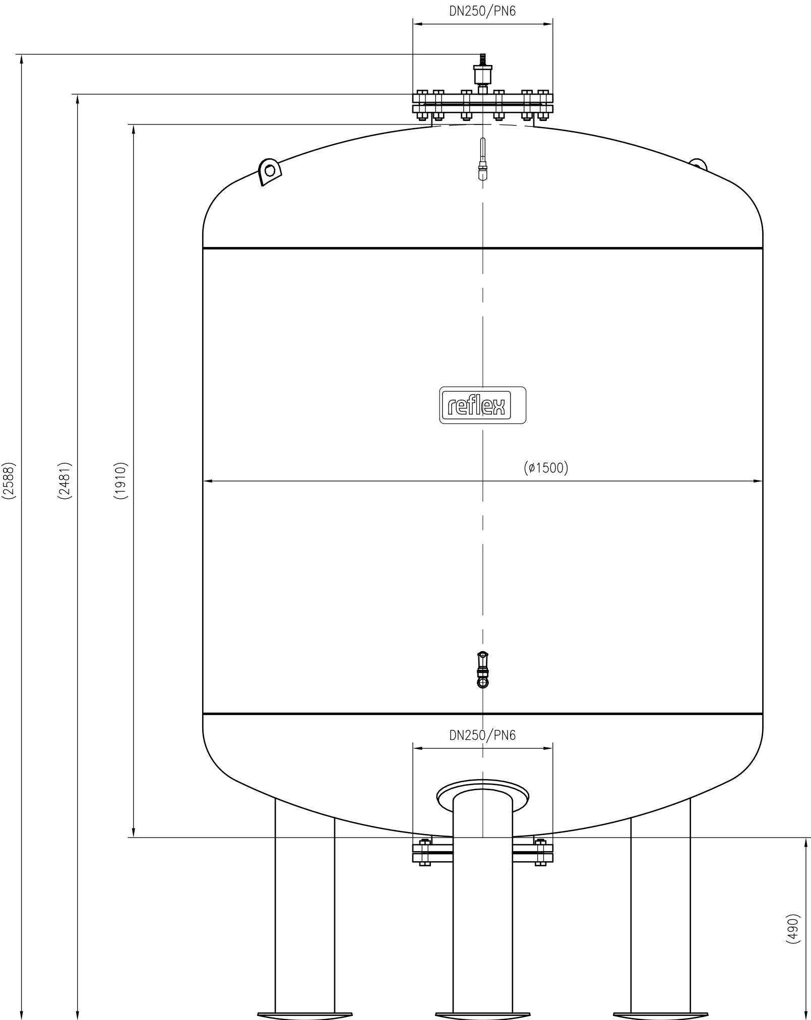
Front view
