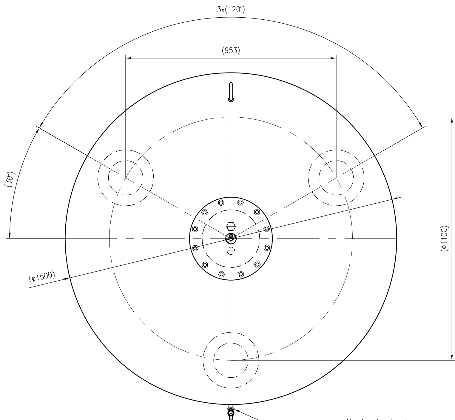
Top view
