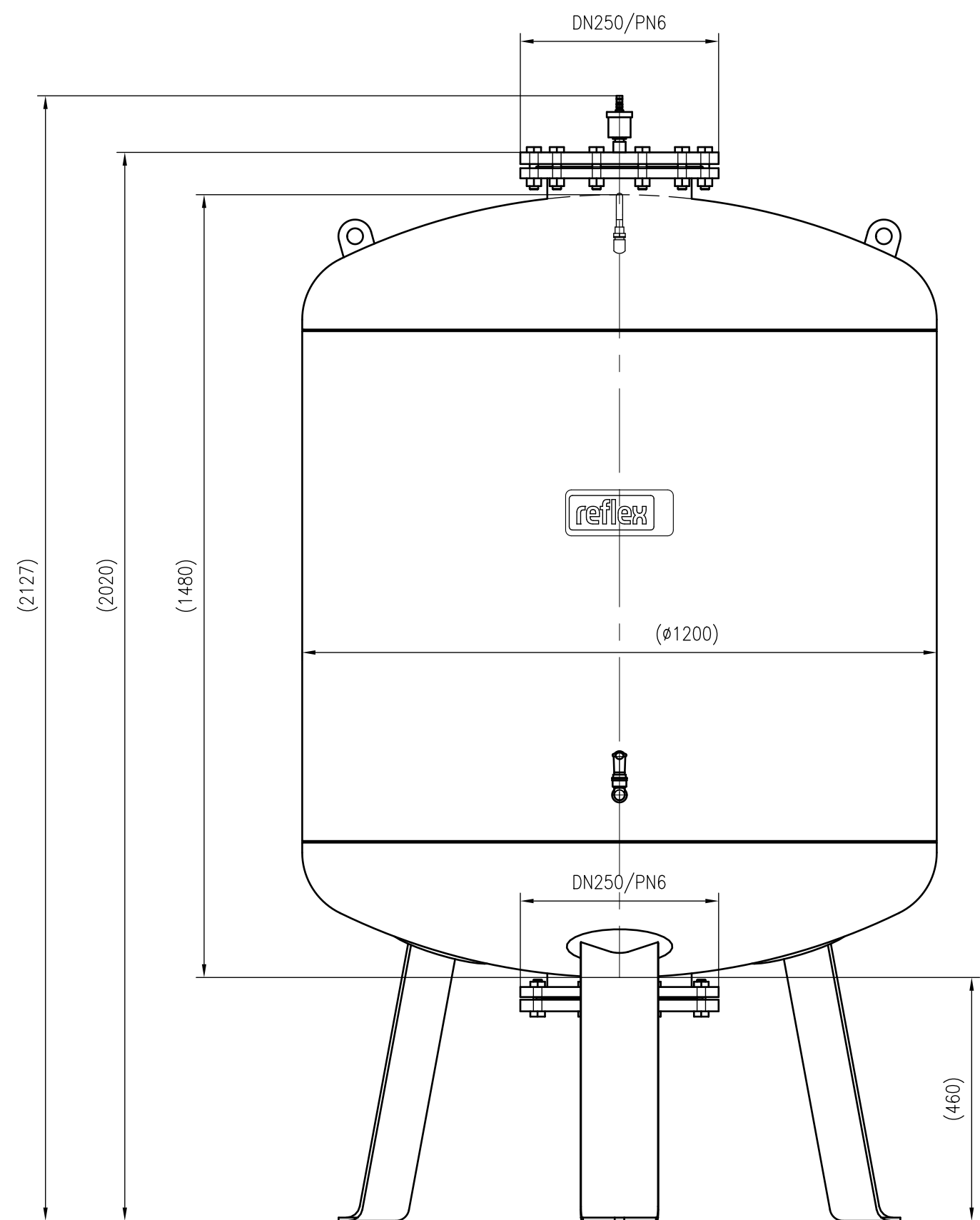
Front view
