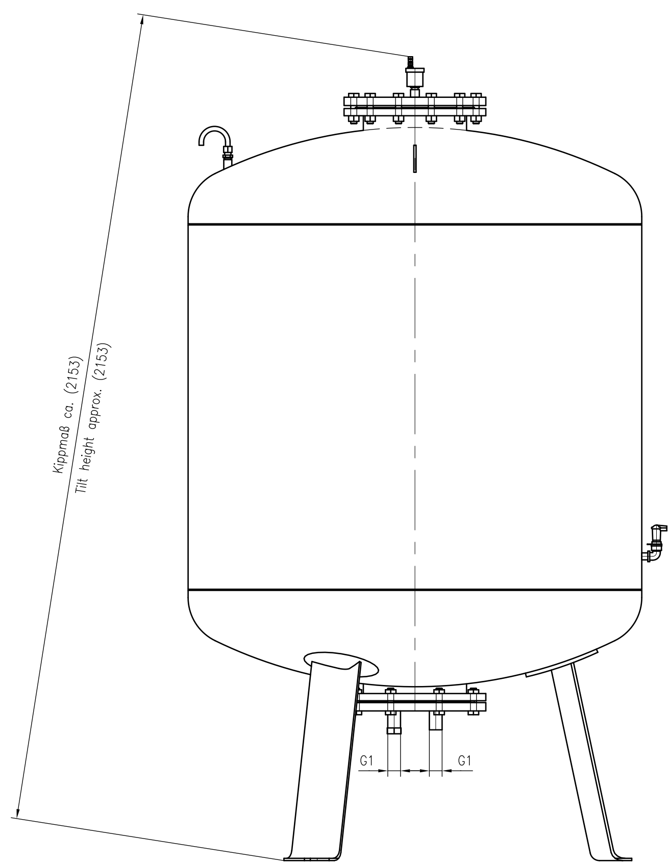
Side view
