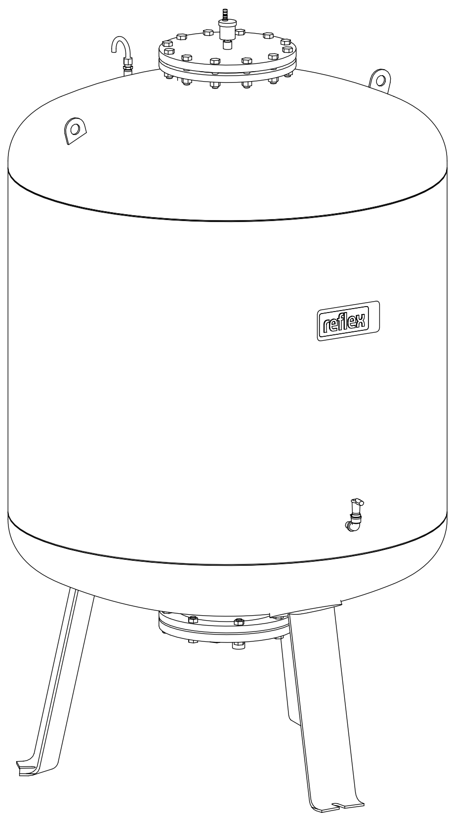
Isometric view
