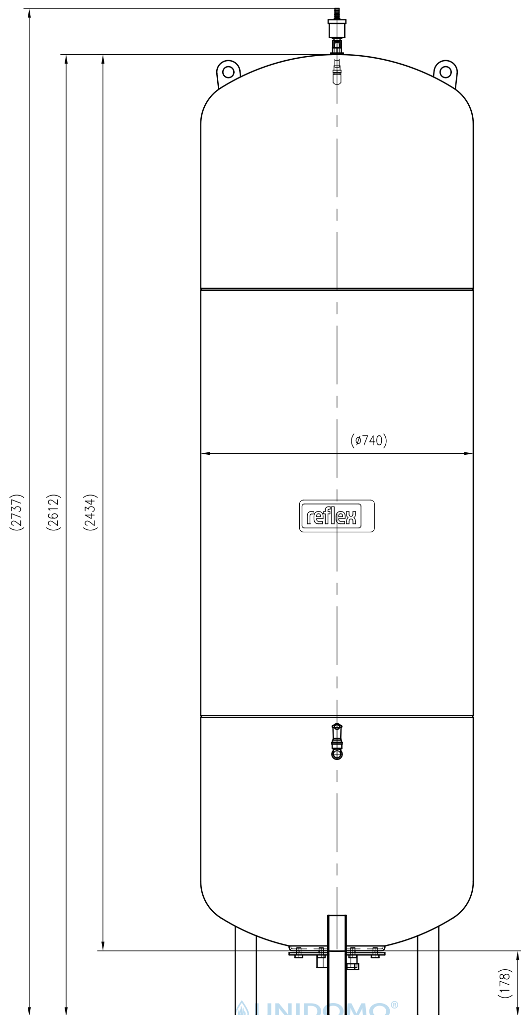
Front view
