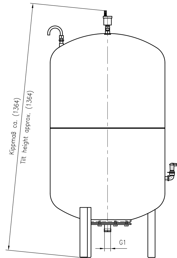
Side view
