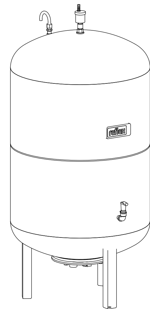
Isometric view
