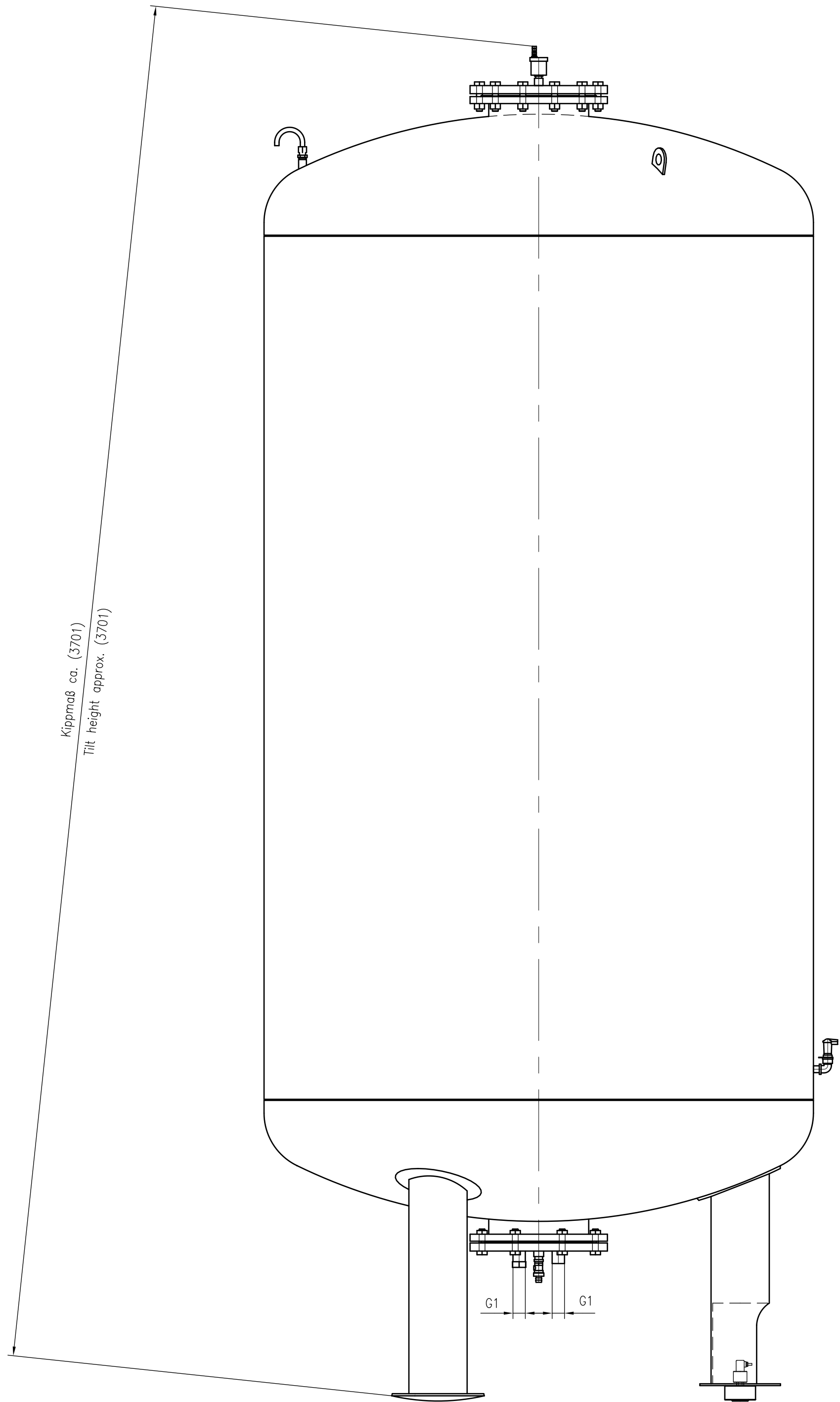
Side view
