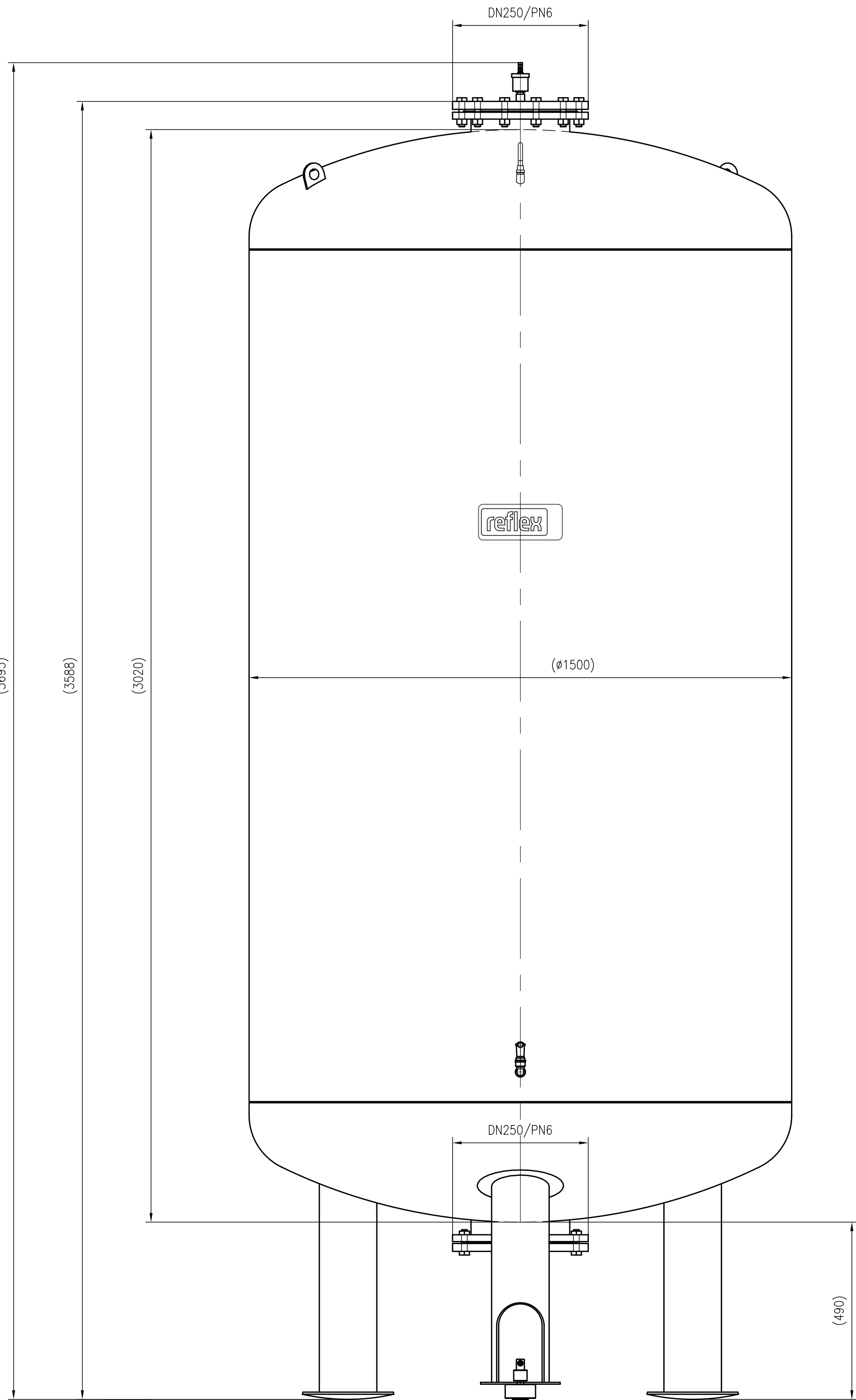
Front view
