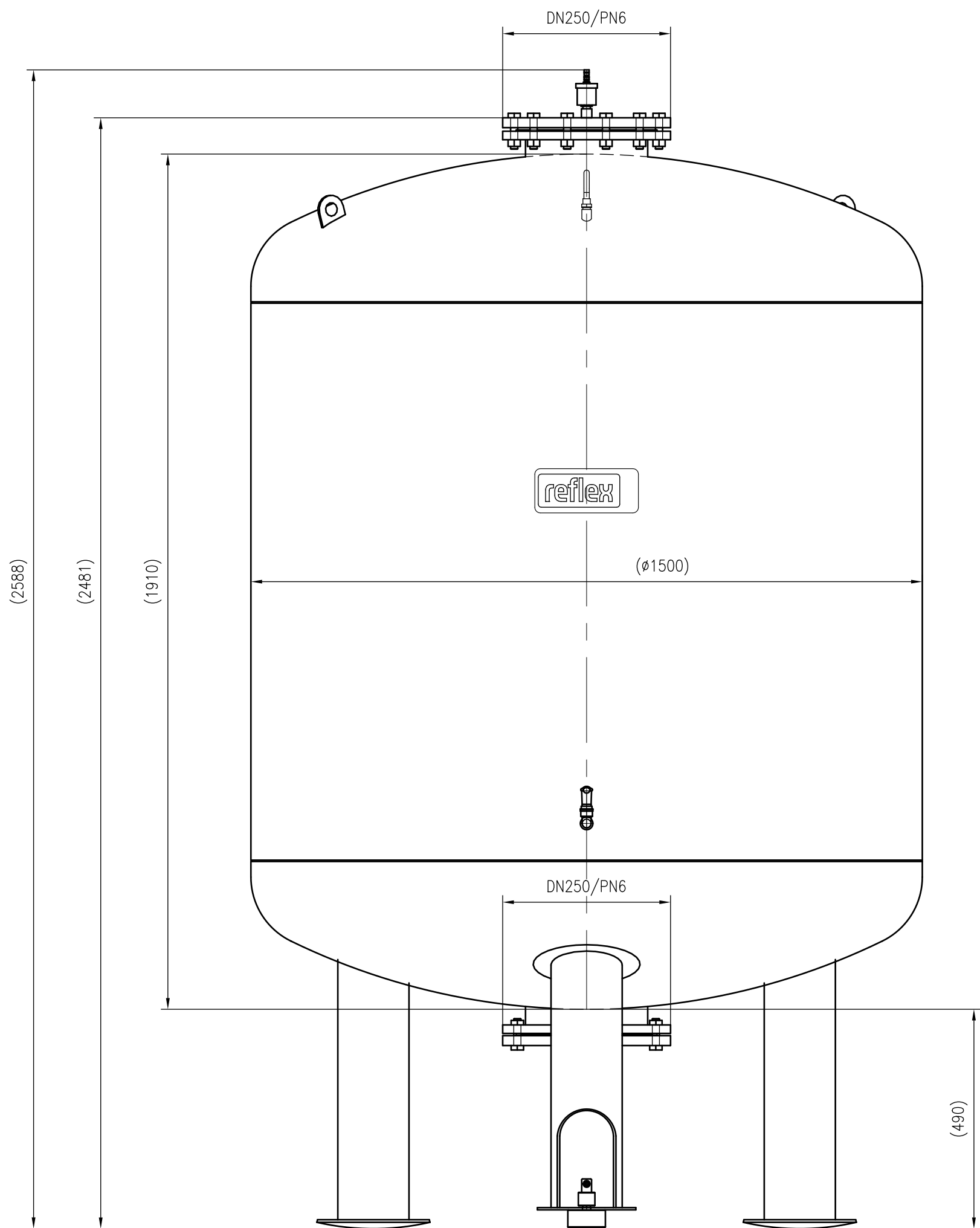
Front view
