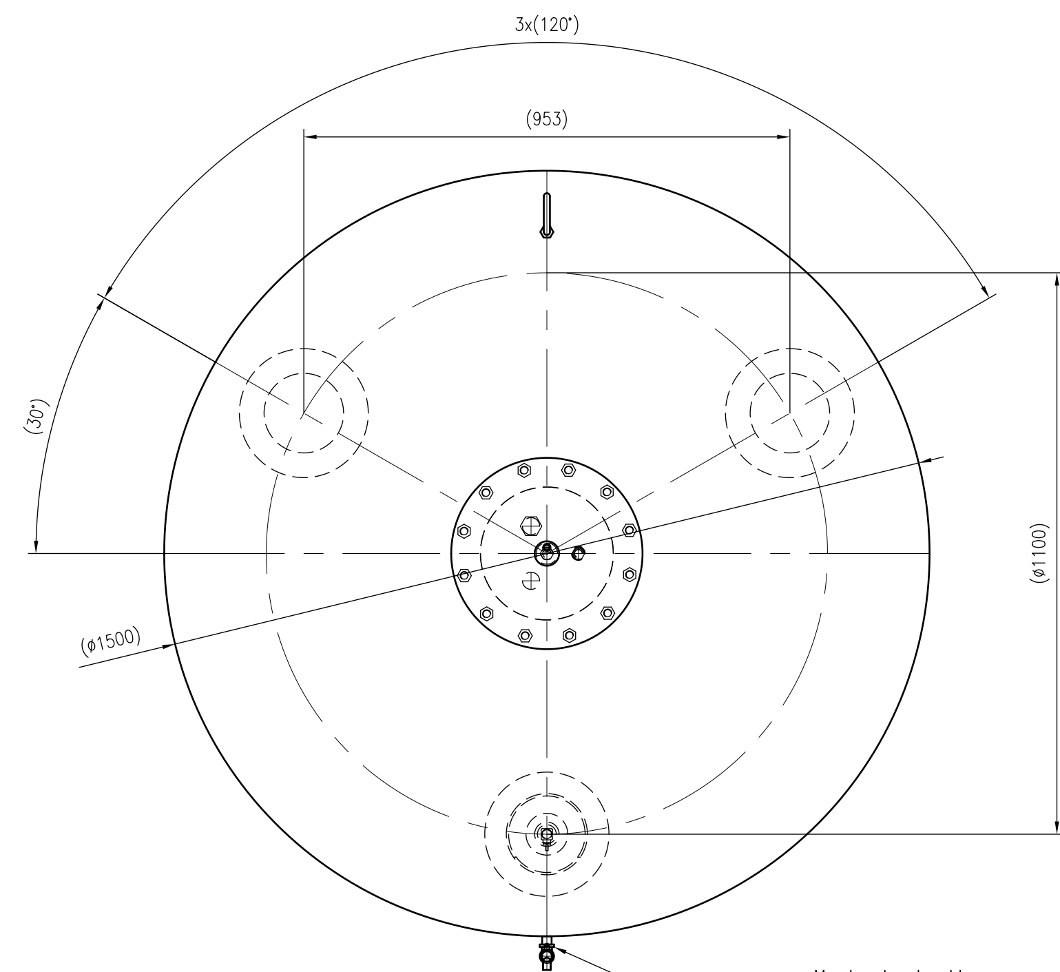
Top view
