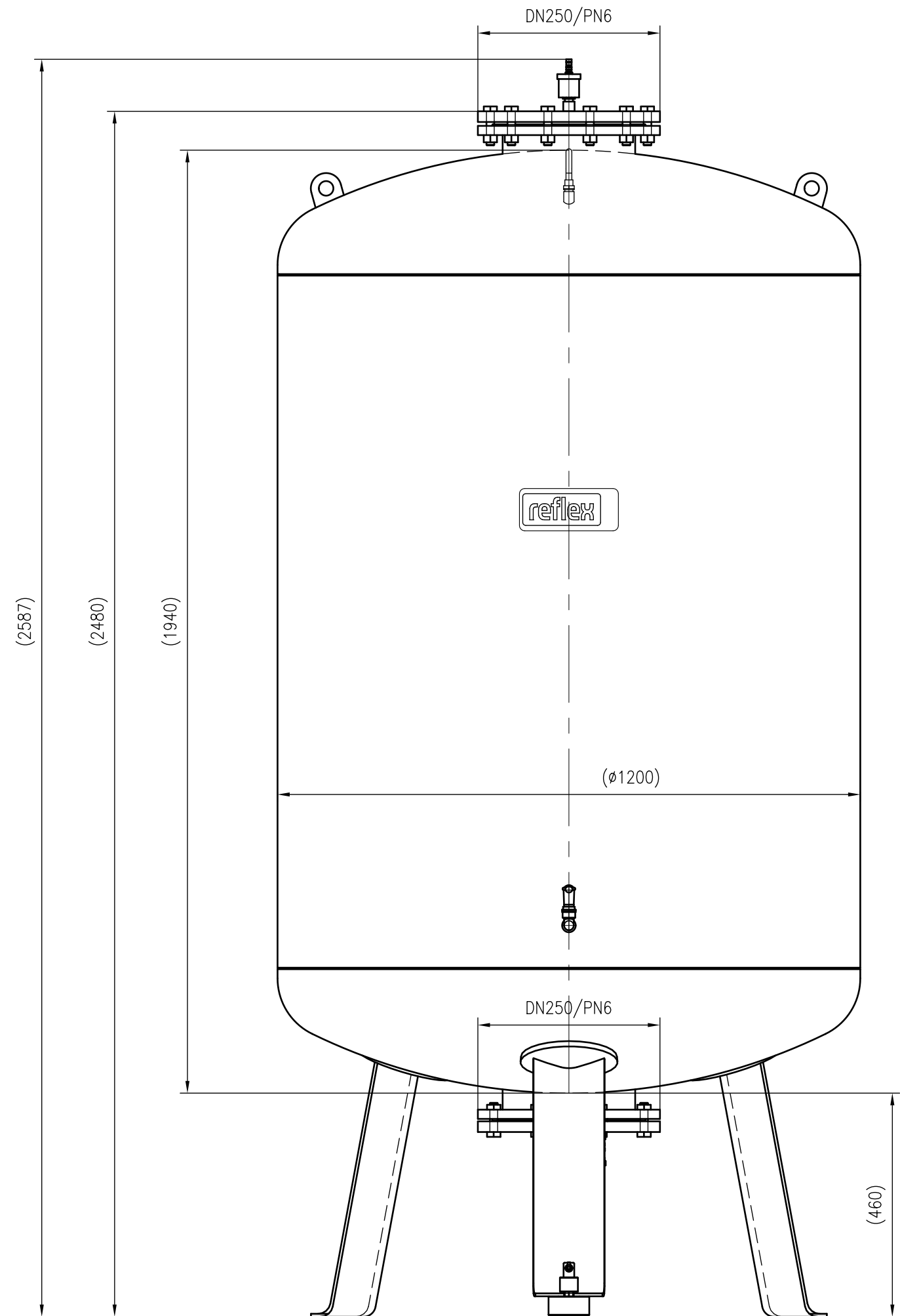
Front view
