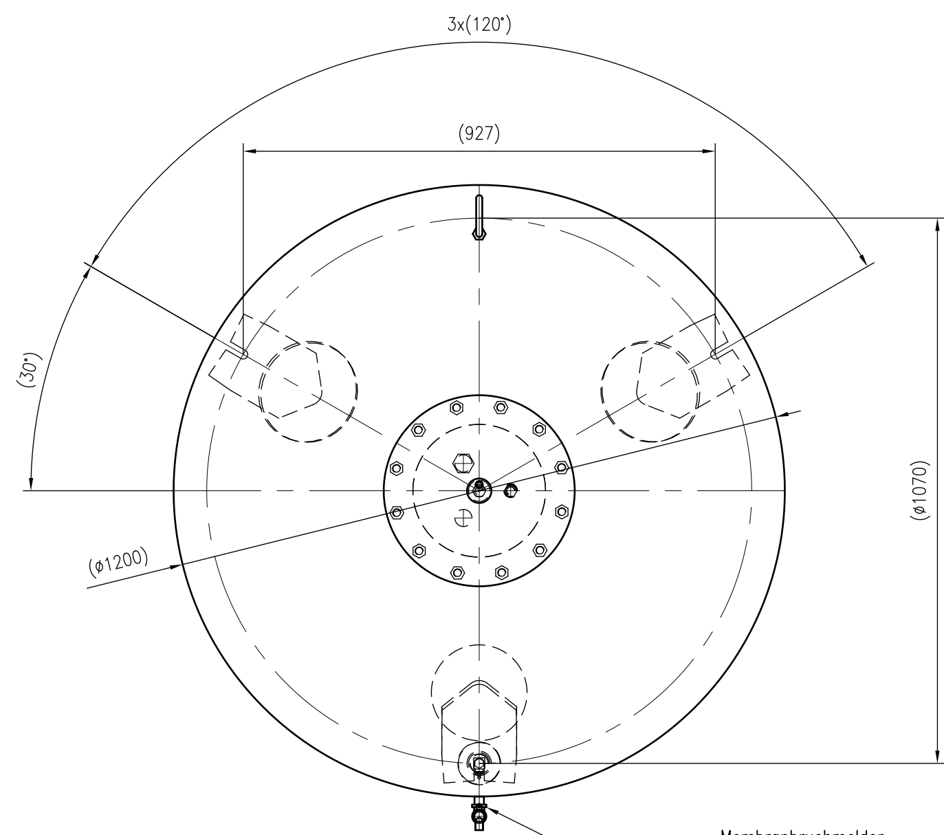
Top view
