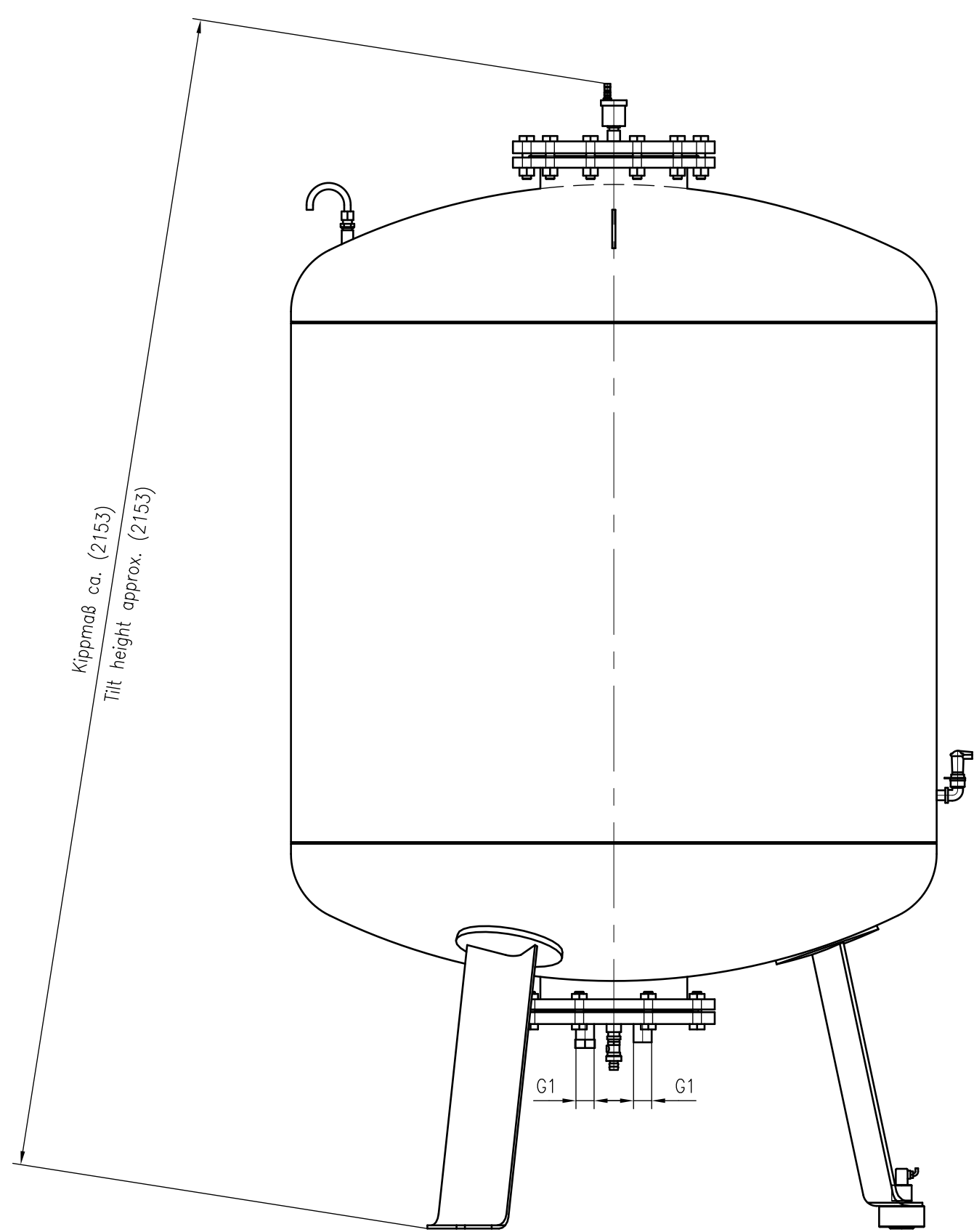
Side view
