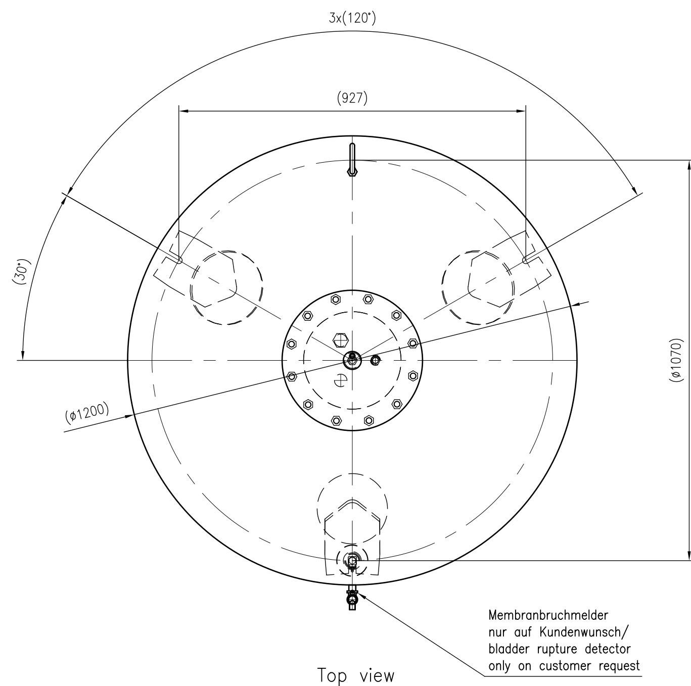
Top view
