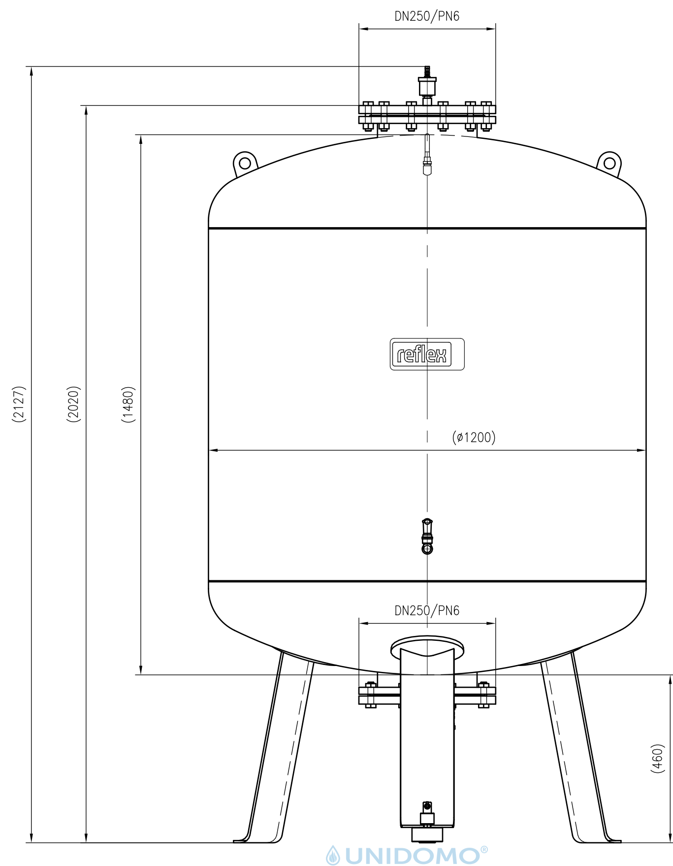
Front view
