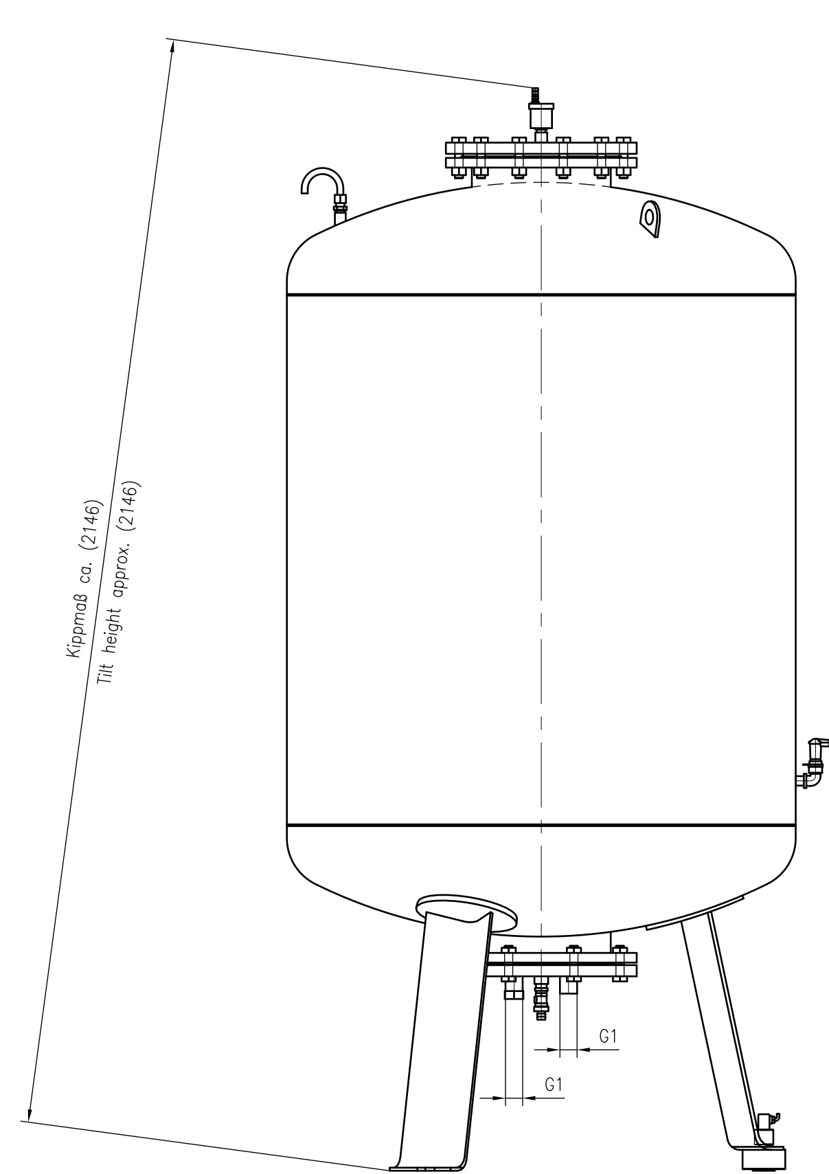
Side view
