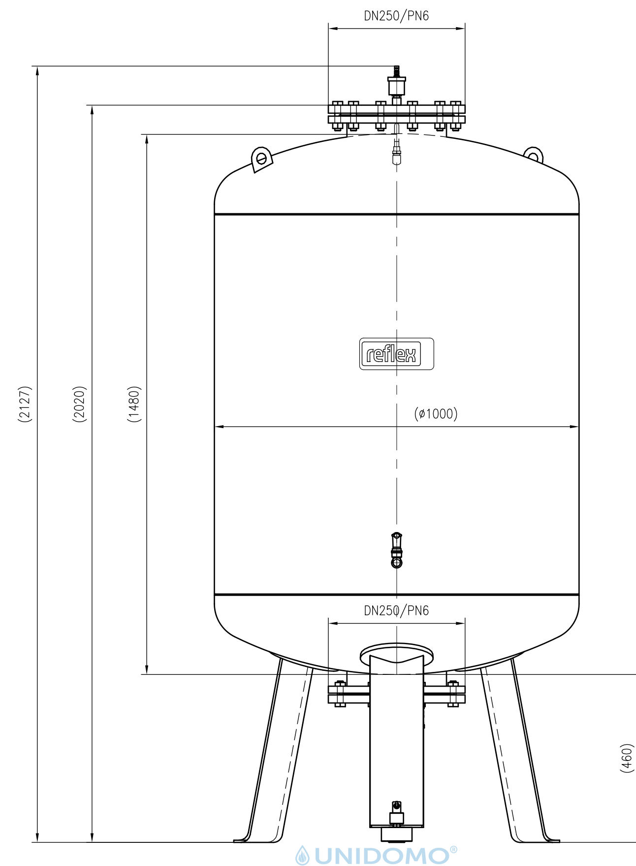
Front view
