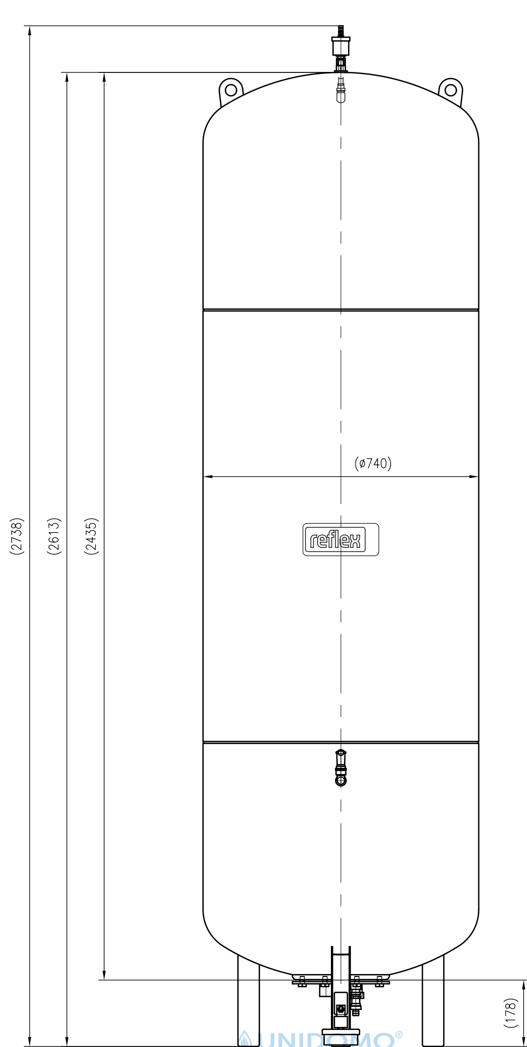
Front view
