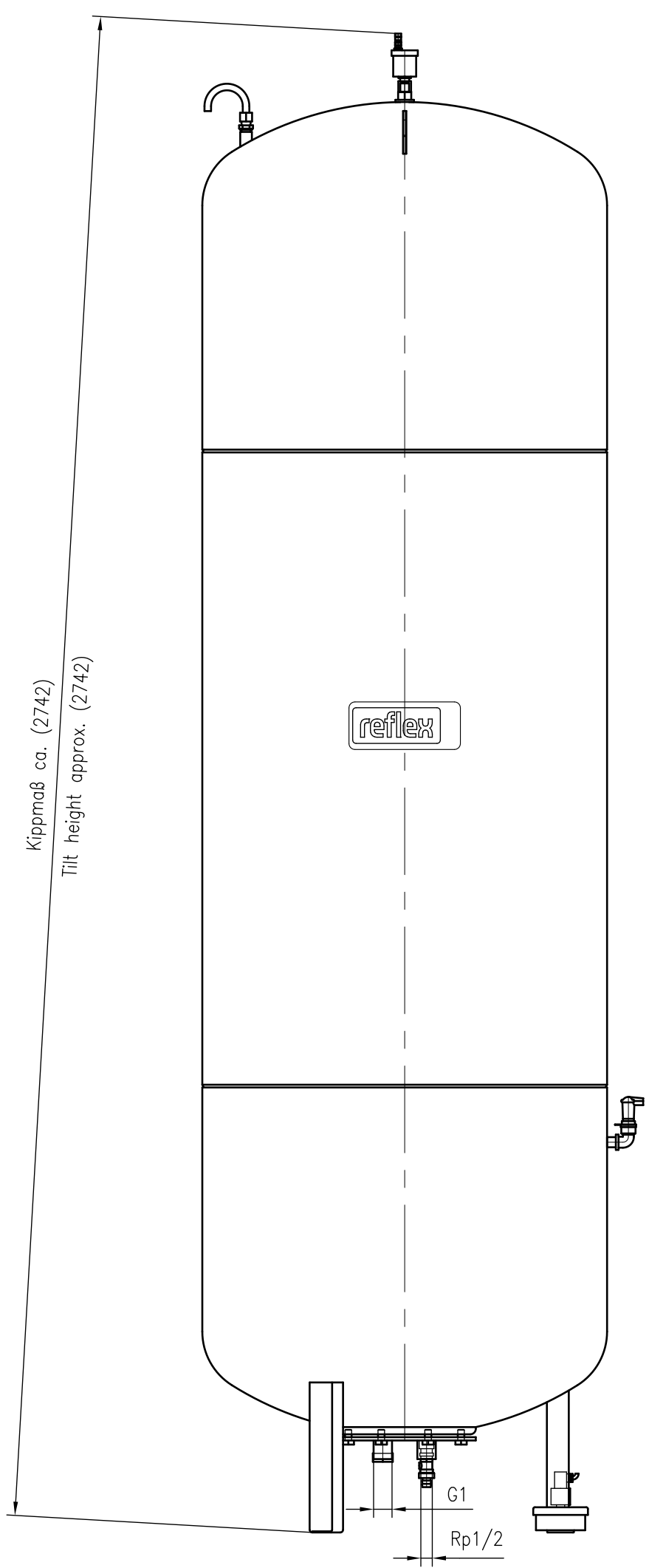
Side view
