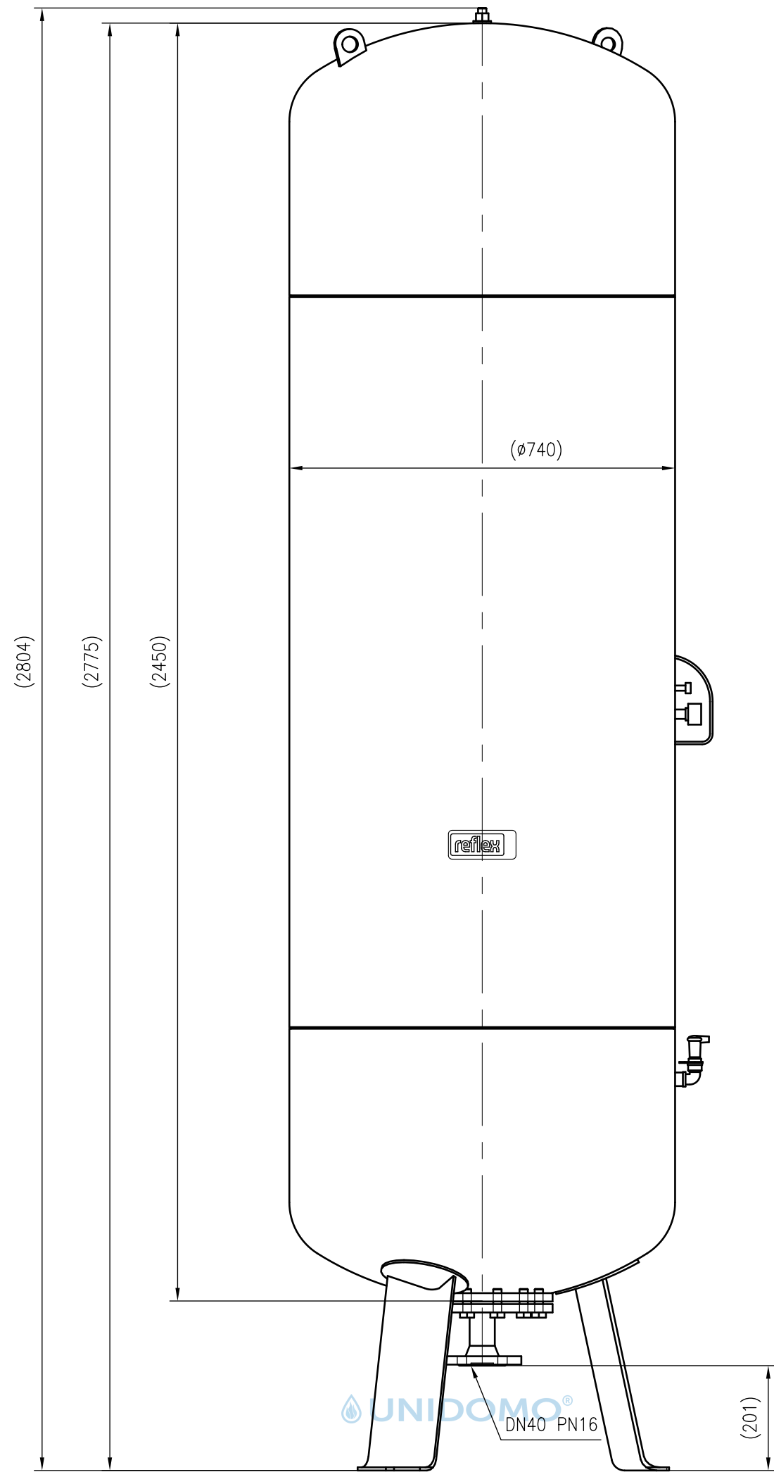
Front view
