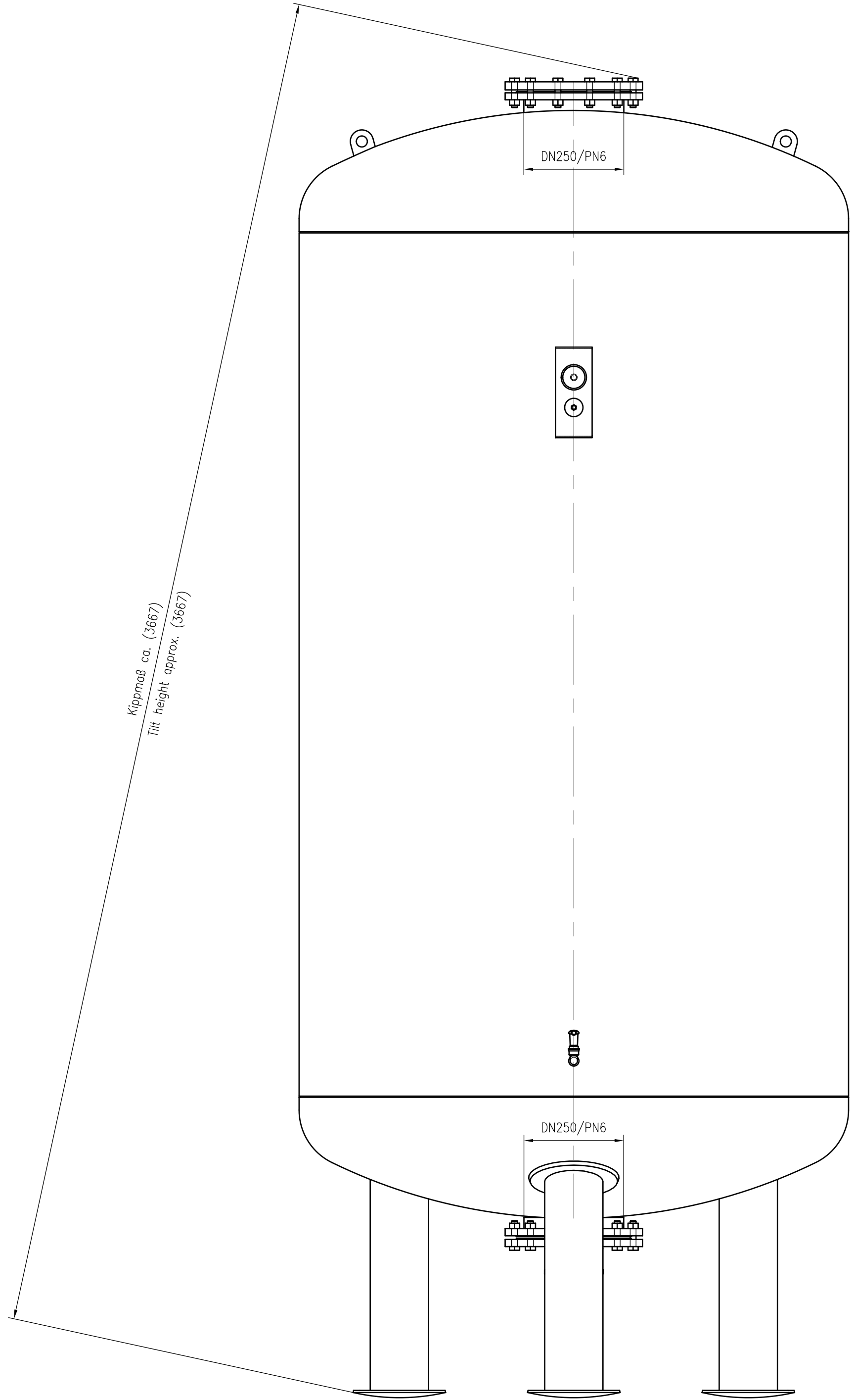
Side view
