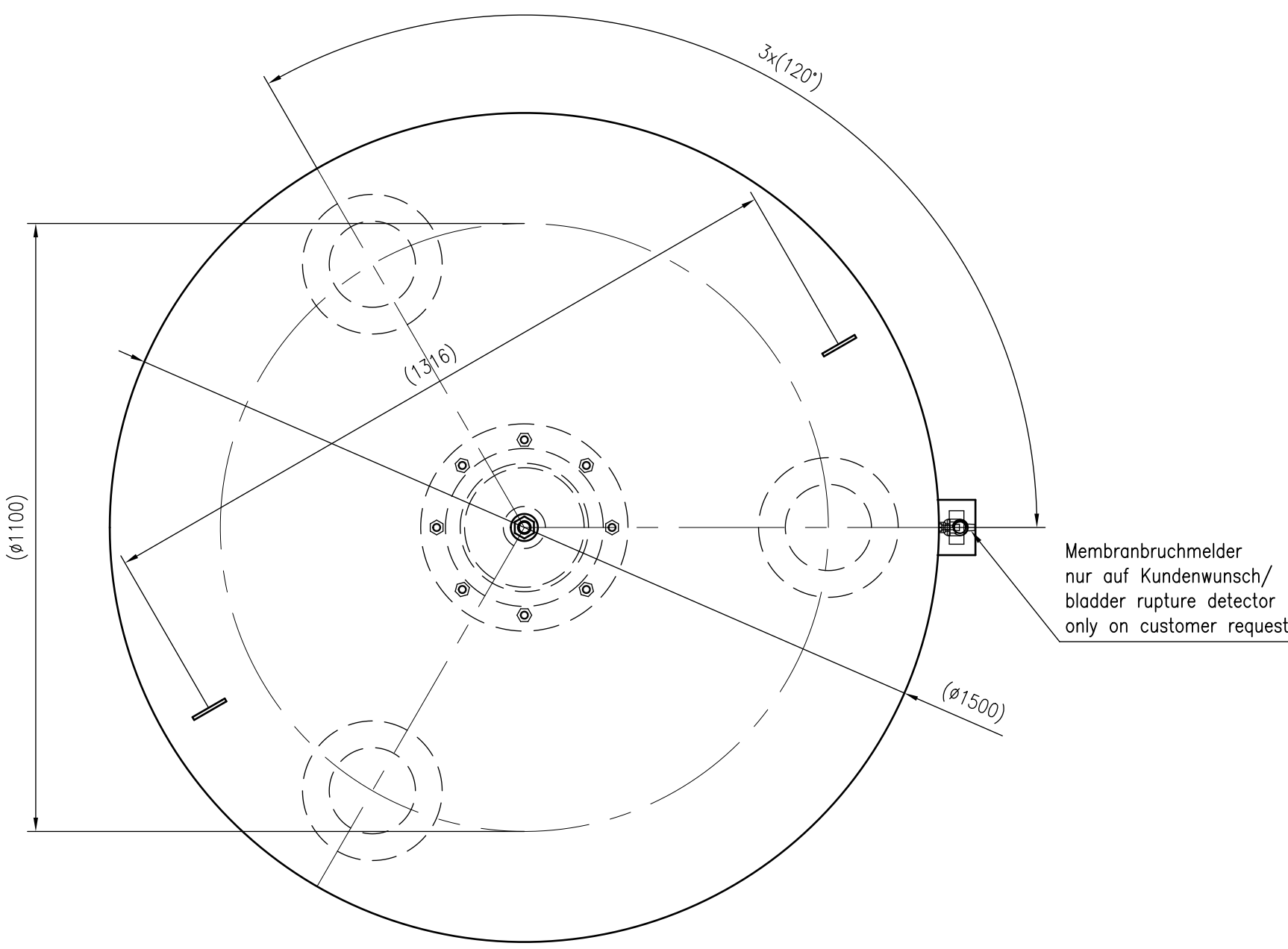
Top view
