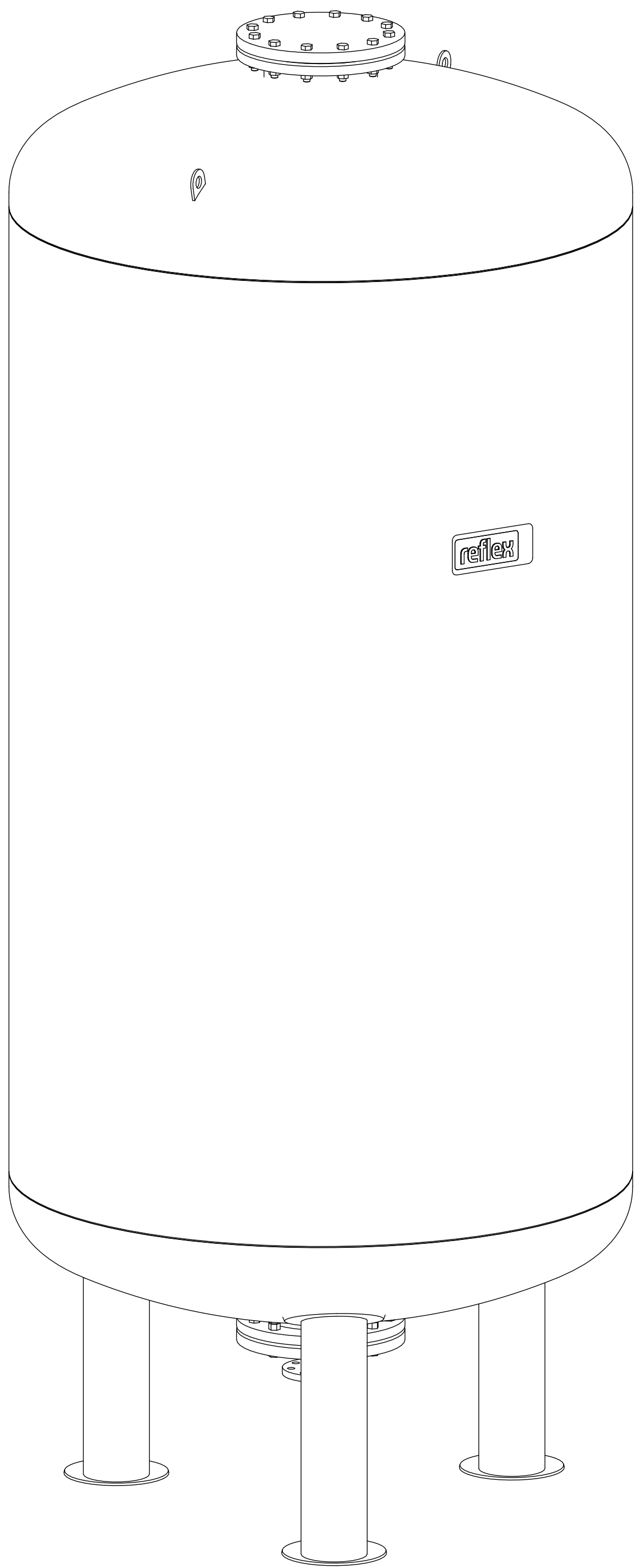
Isometric view
