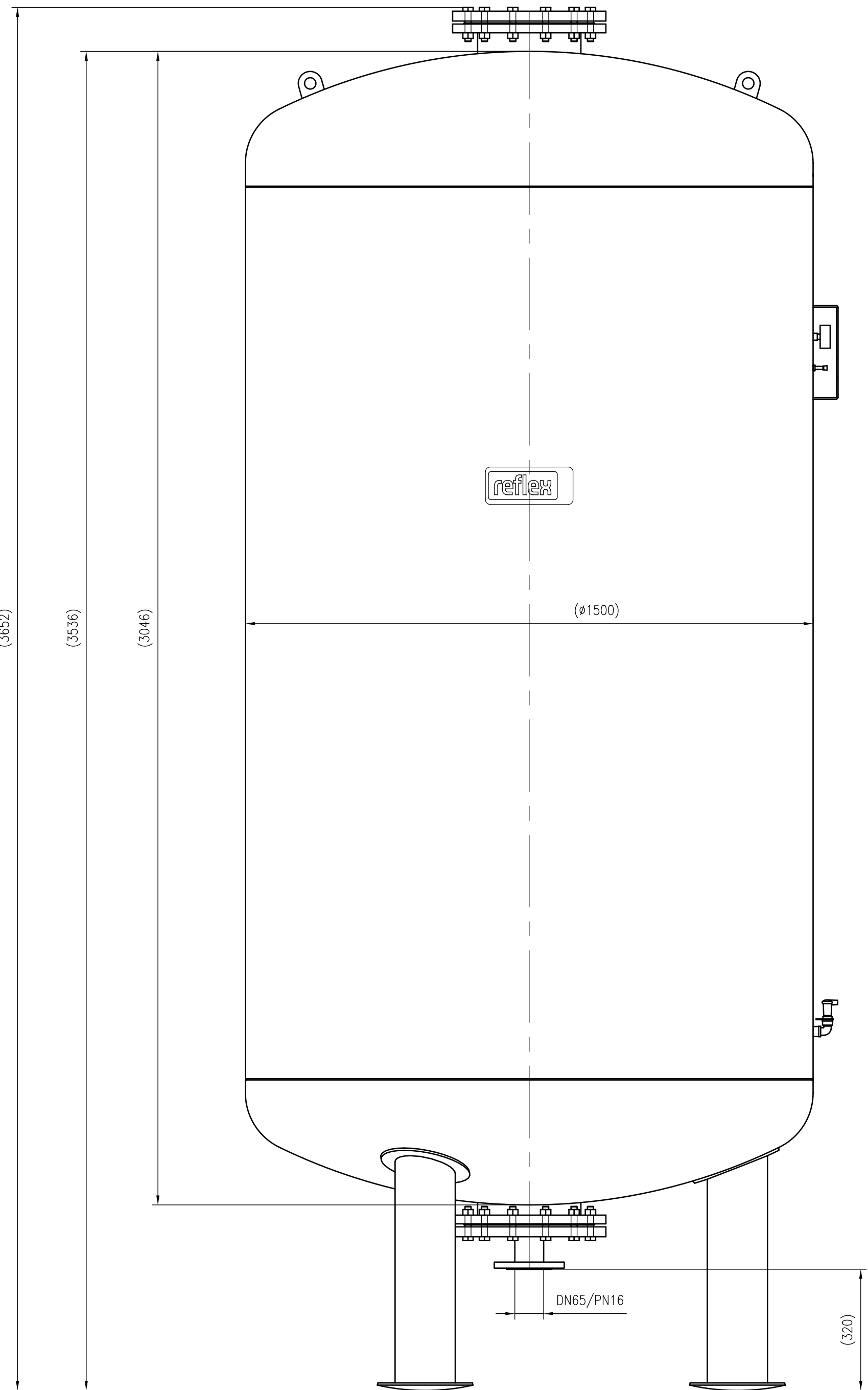
Front view
