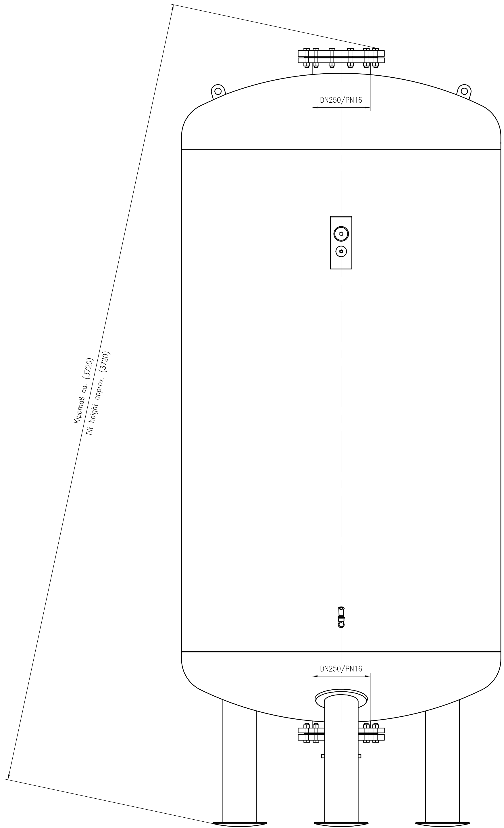
Side view
