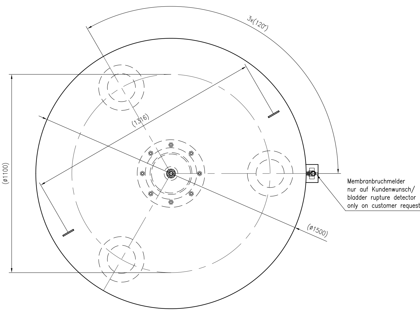
Top view
