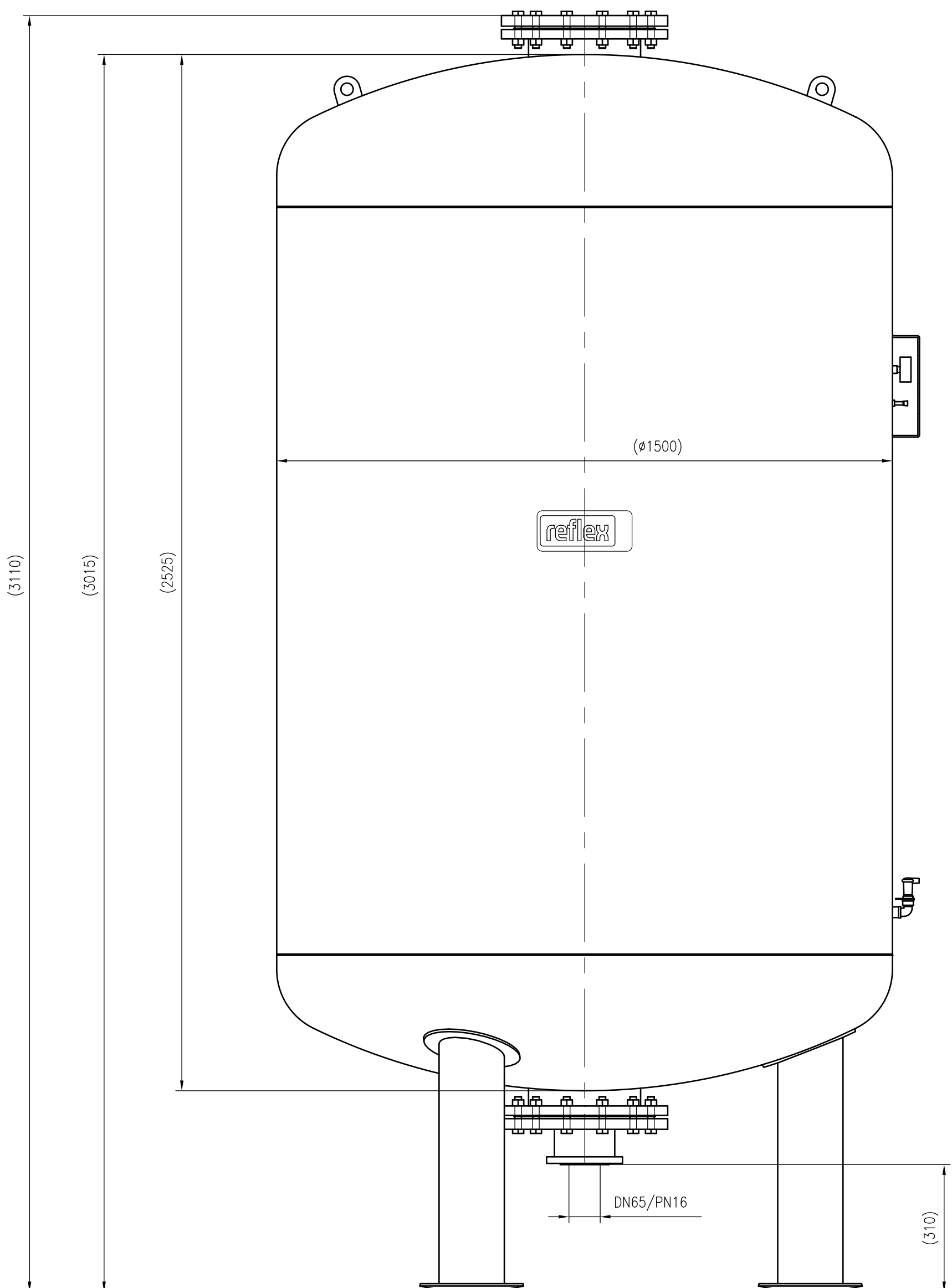
Front view
