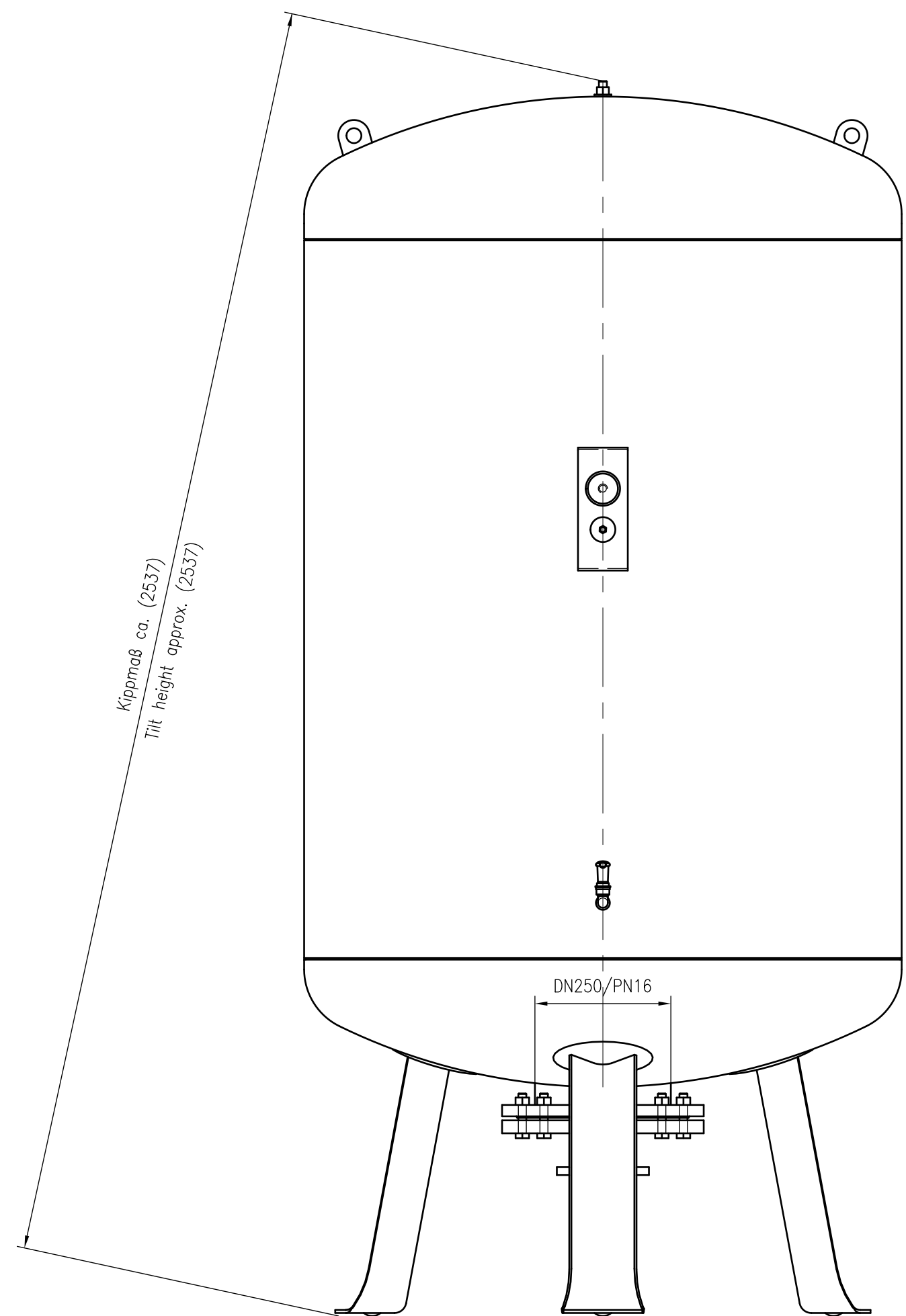
Side view
