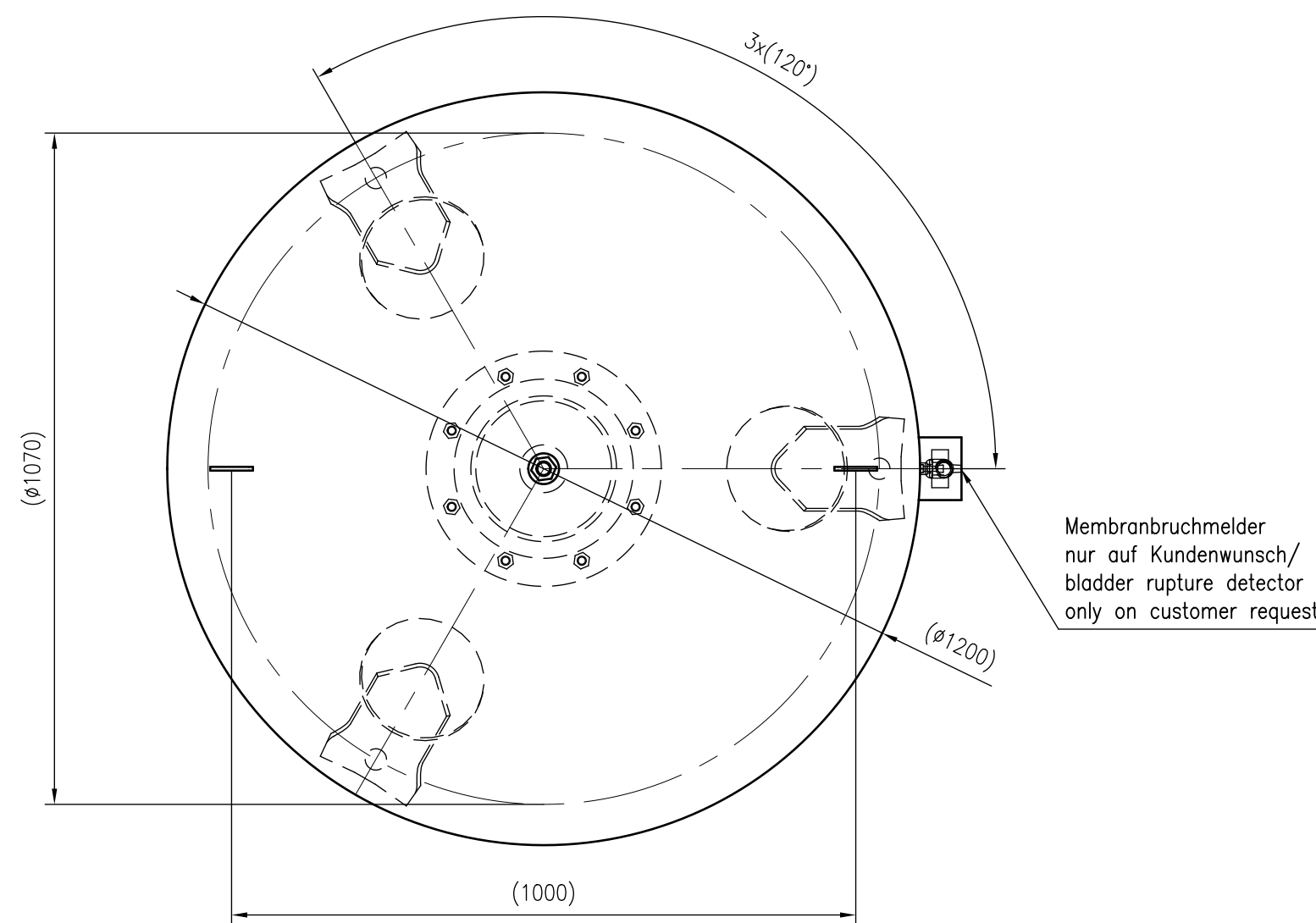
Top view
