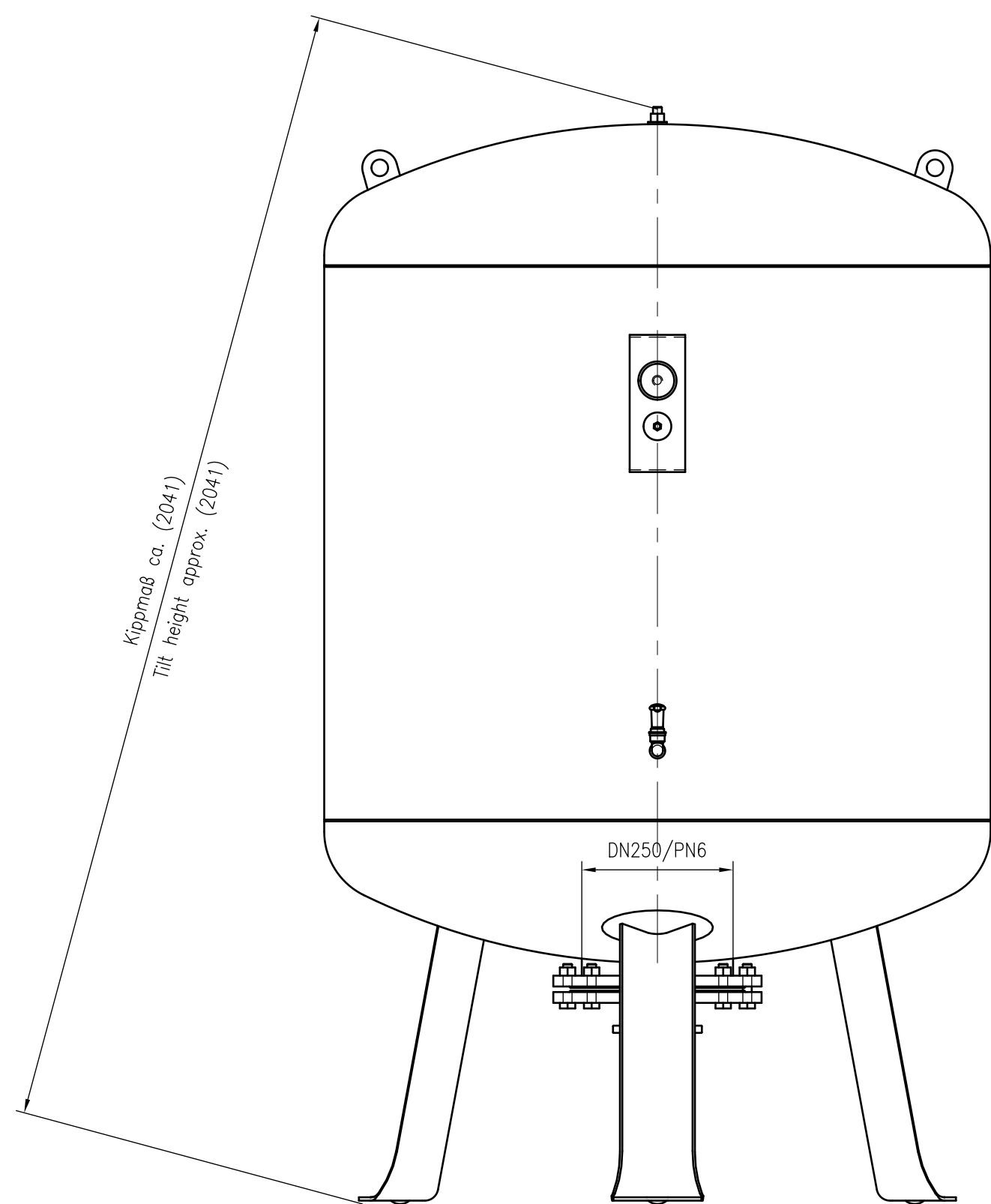
Side view
