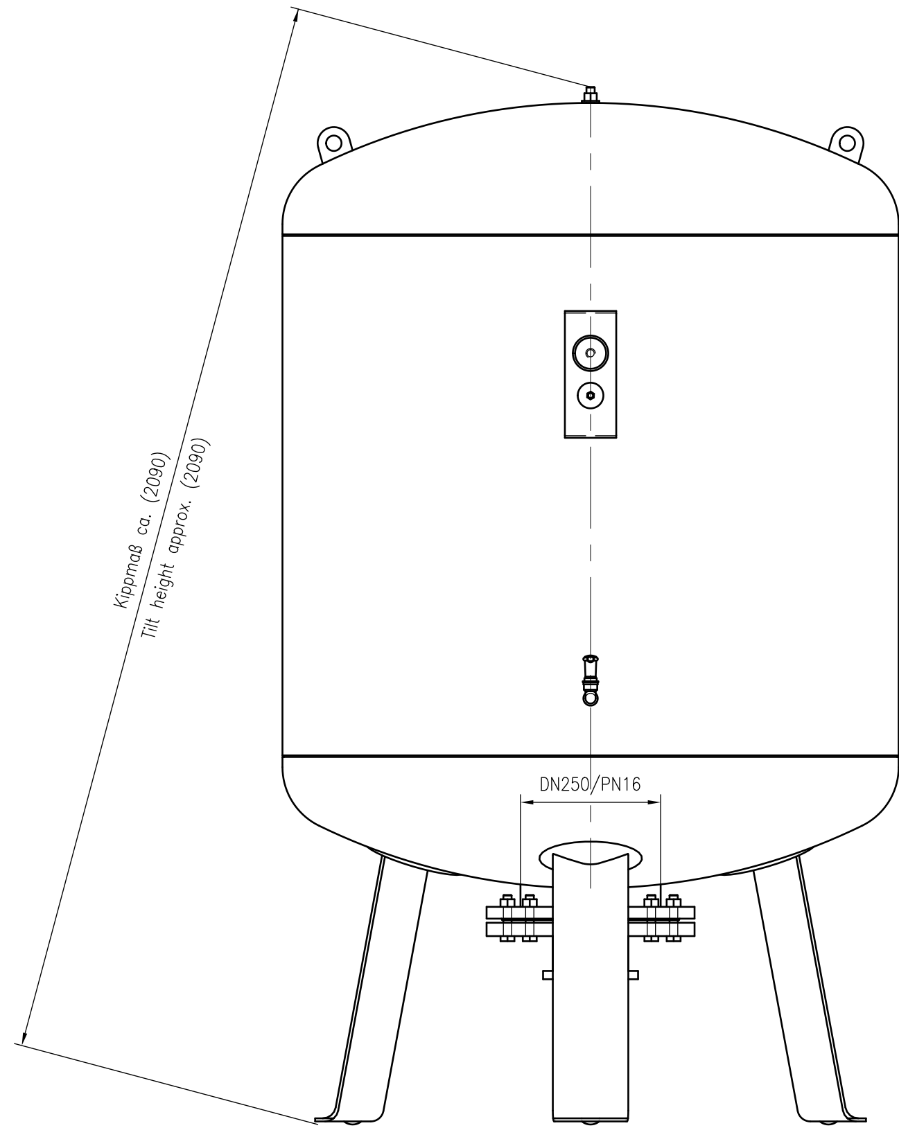
Side view
