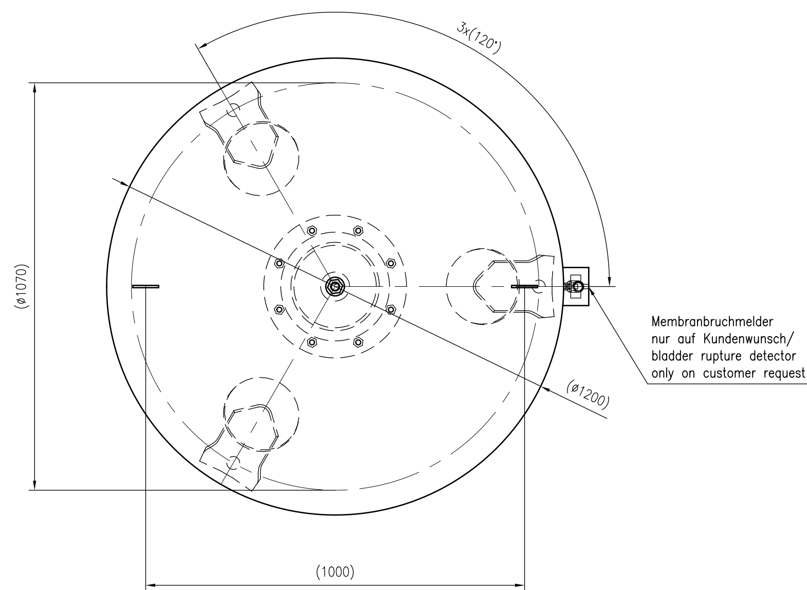
Top view
