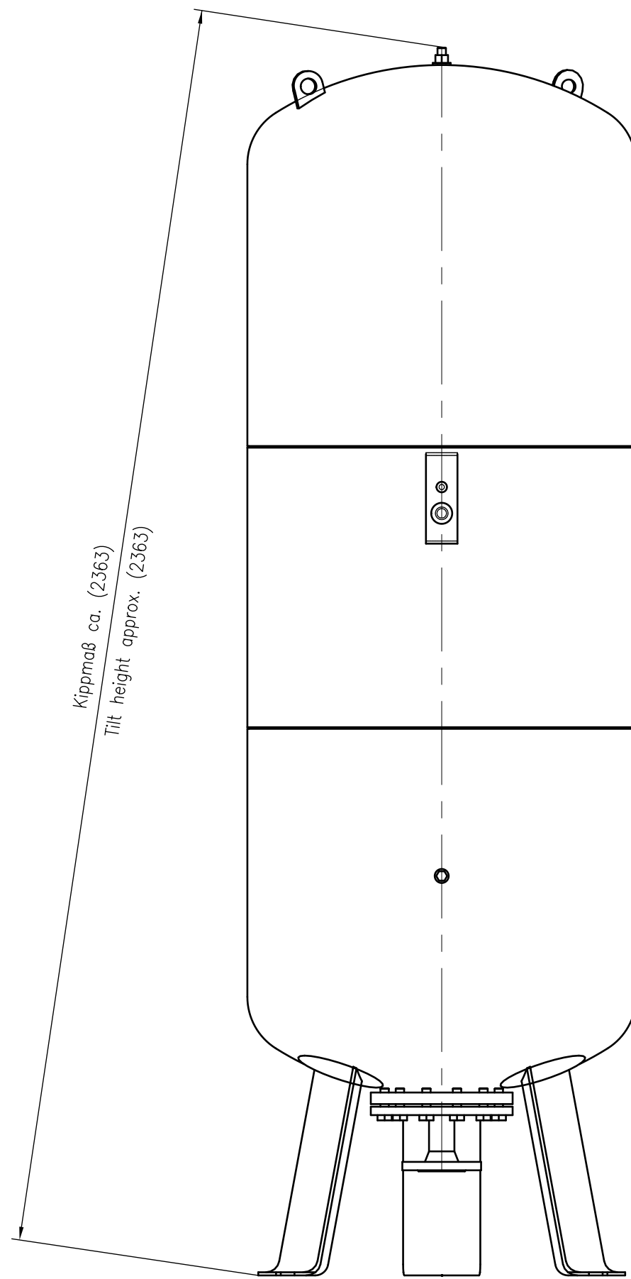
Side view
