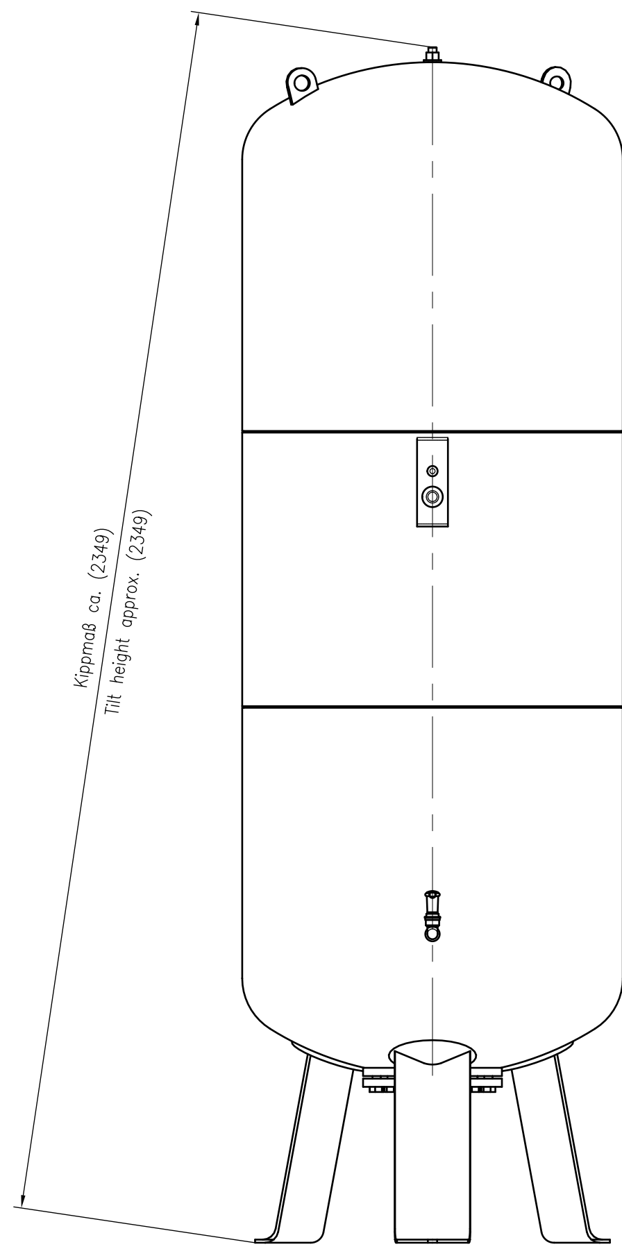
Side view
