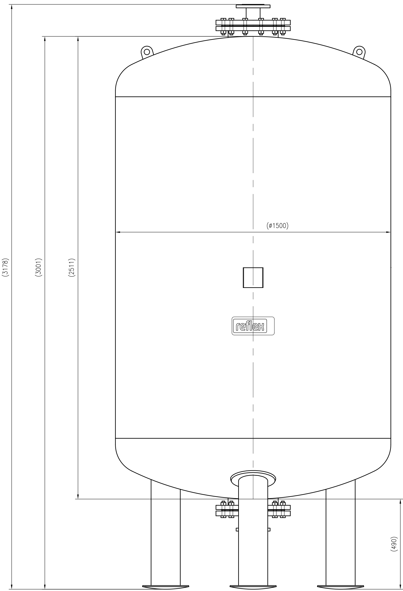
Front view
