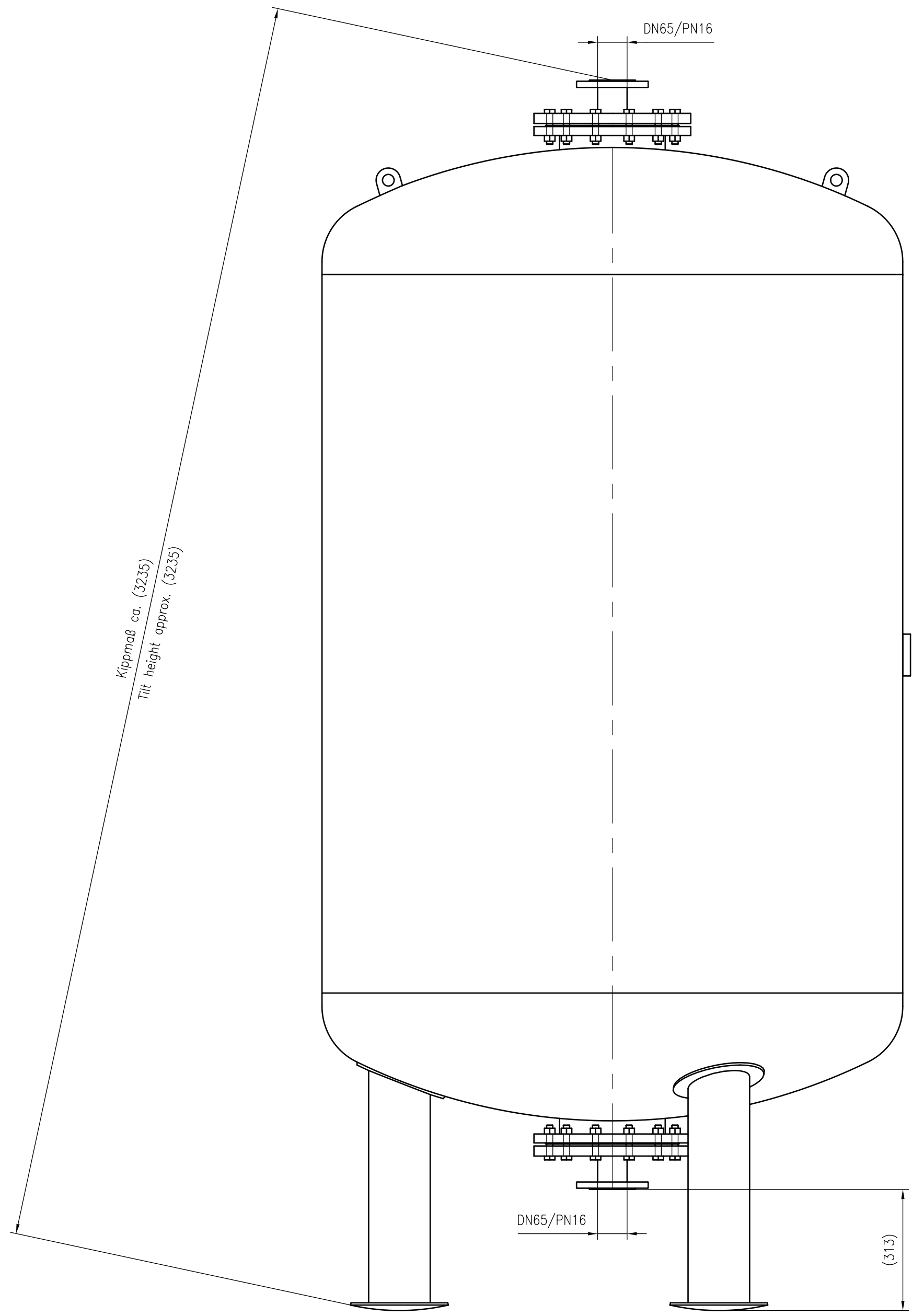
Side view
