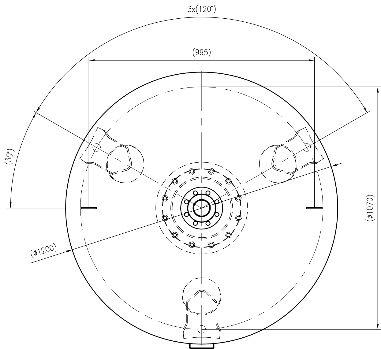
Top view
