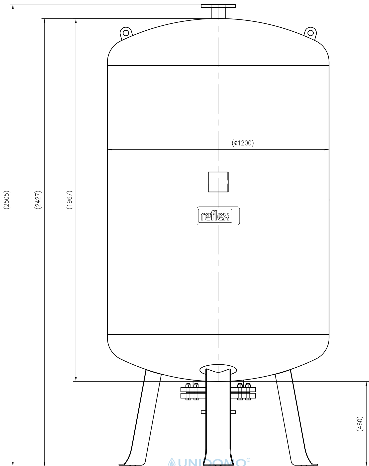
Front view
