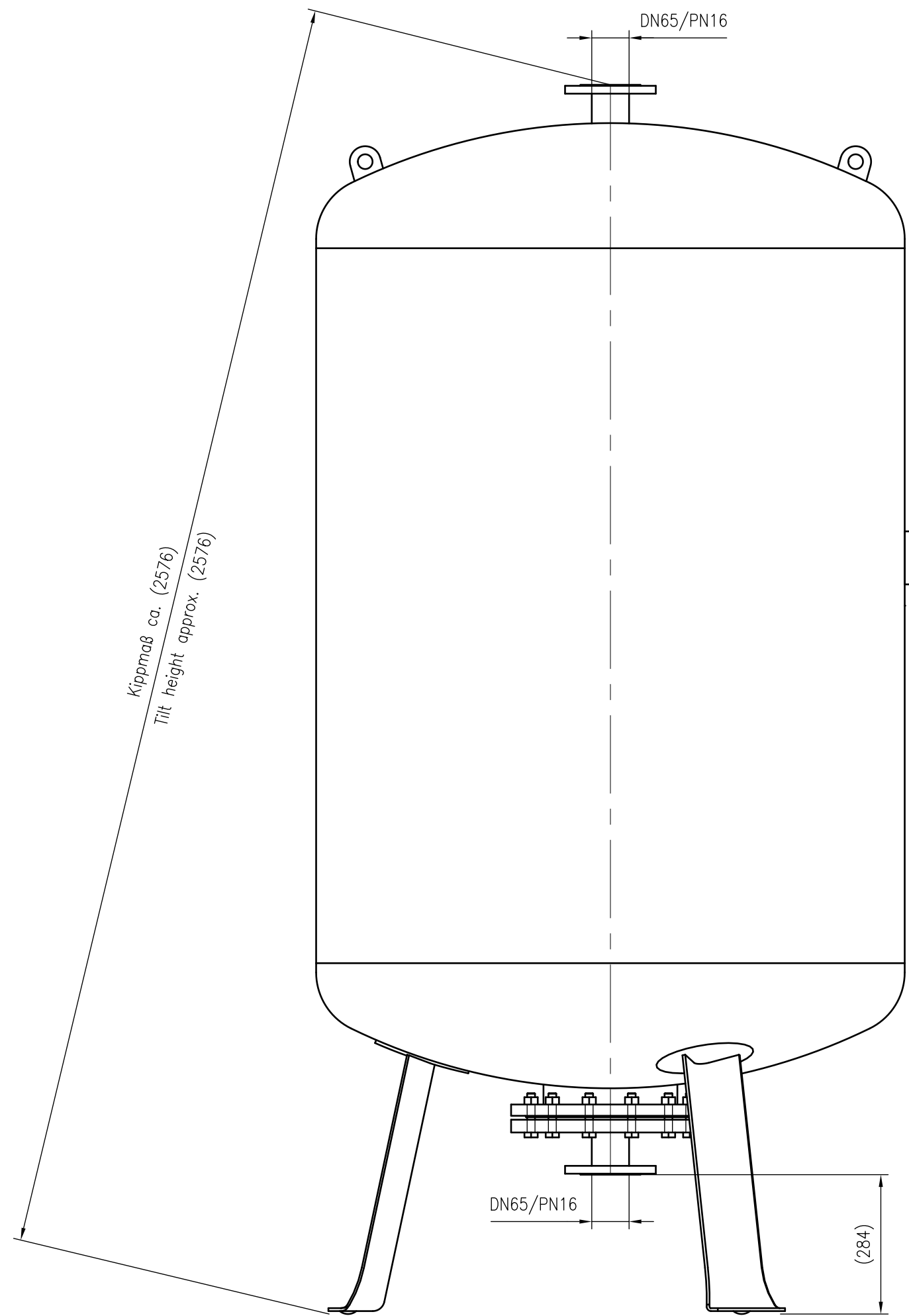
Side view
