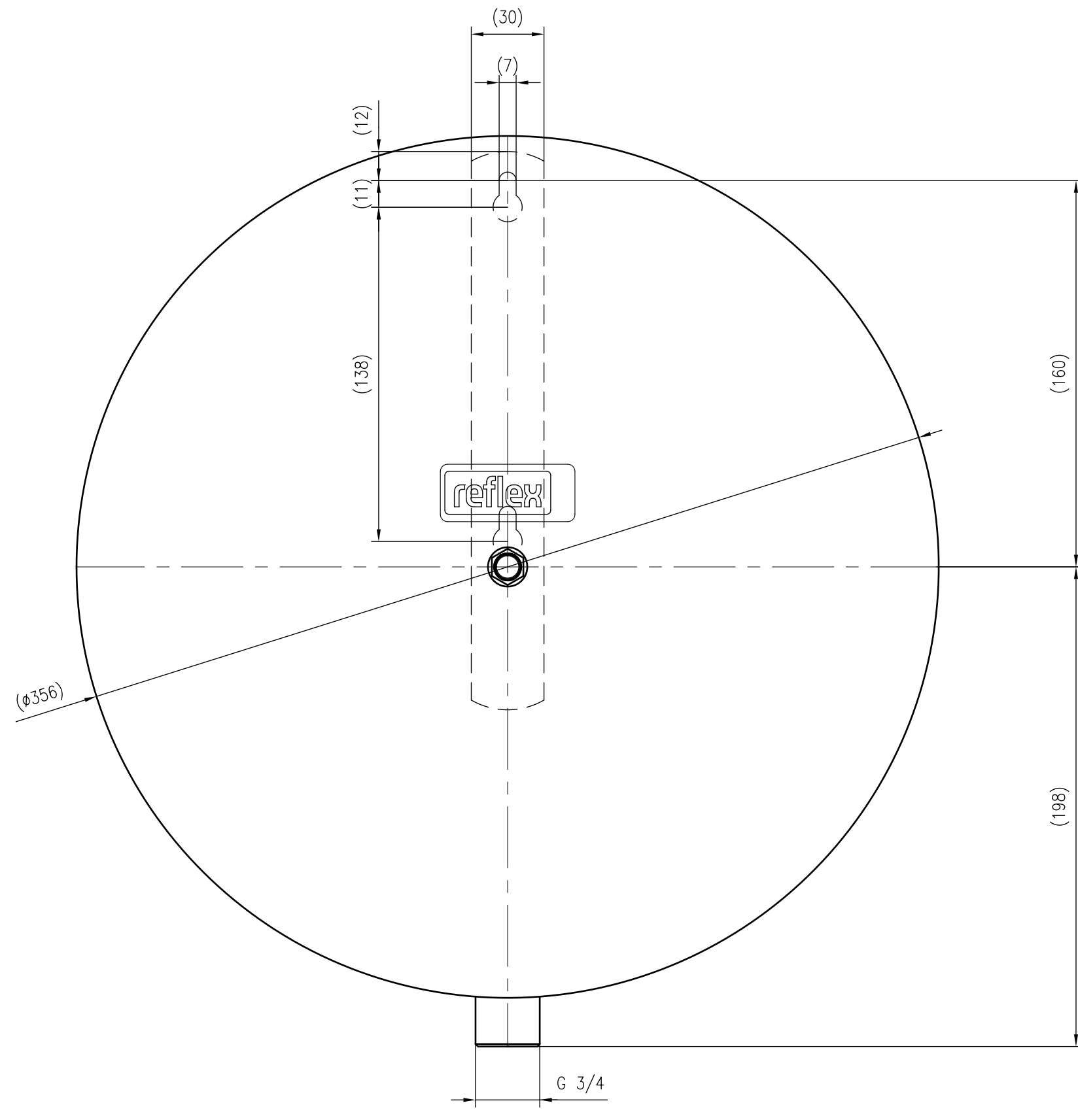
Front view
